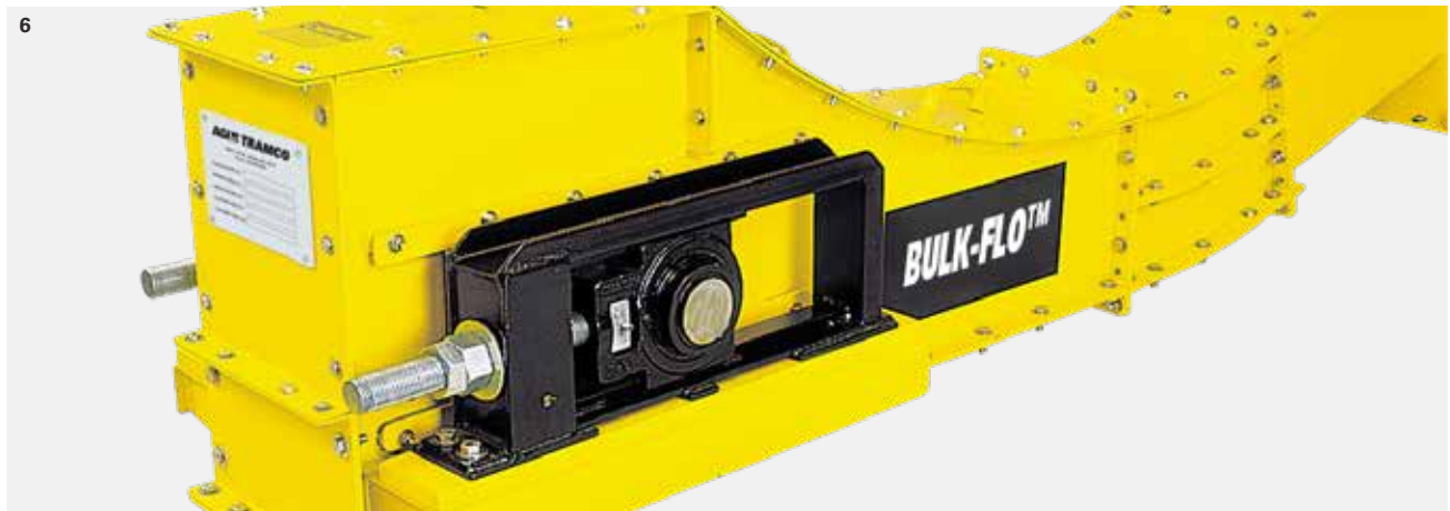
Standard Head (without cover) showing the double-life walking tooth split sprocket
