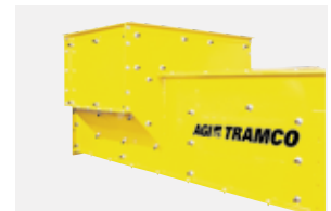
Bypass feed inlet with replaceable abrasion resistant liners and optional feeder boxes also available.
