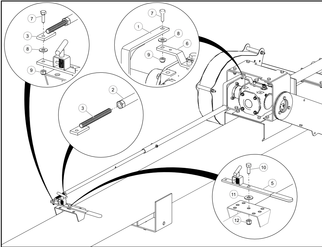
Figure 2 Hole Positions in Straight Gearbox Handle Extension
