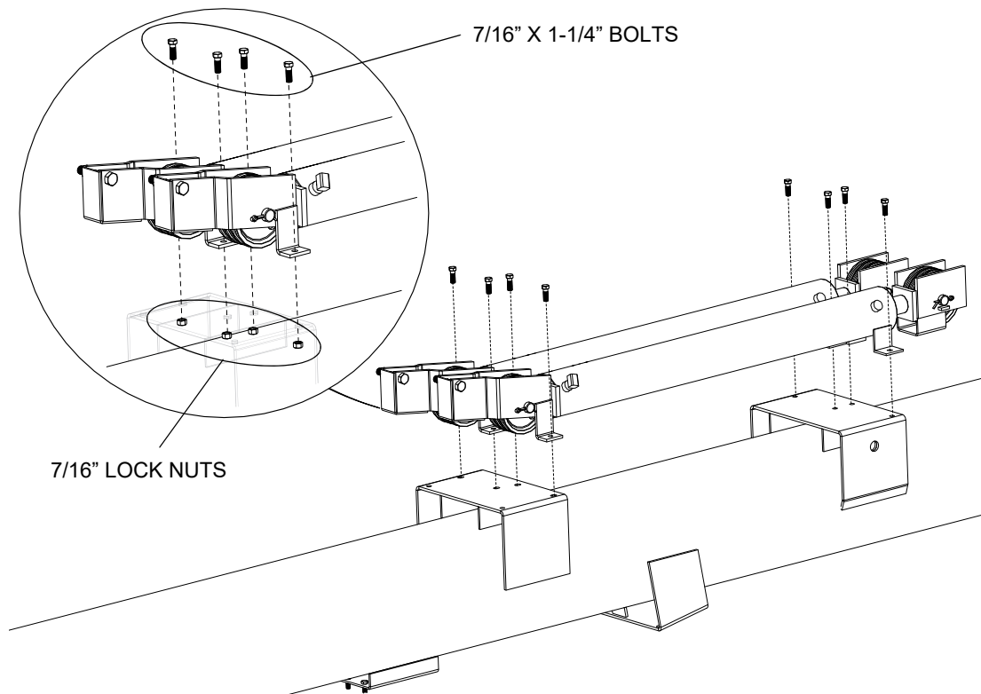
Figure 3. Installing Lift Cylinders
