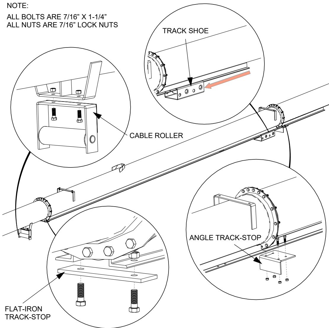
Figure 5. Track Shoe, Cable Roller, and Track-Stop (64' Model)
