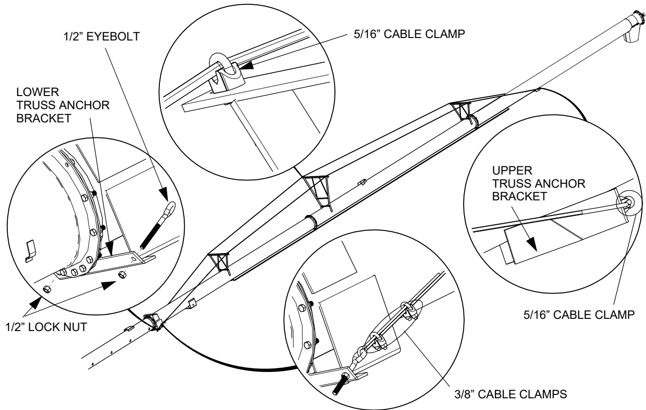
Figure 10. Truss Cables (74' Model)
