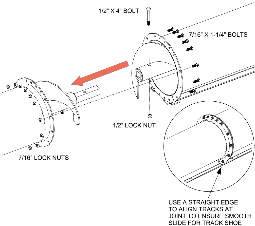
Figure 4. Connecting Auger Tubes Sections and Flights
