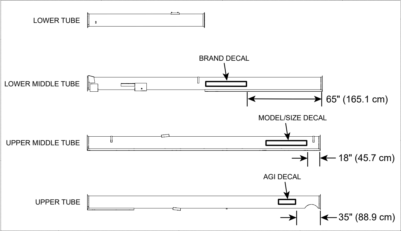
Figure 2. 74' Auger Tube Sections
