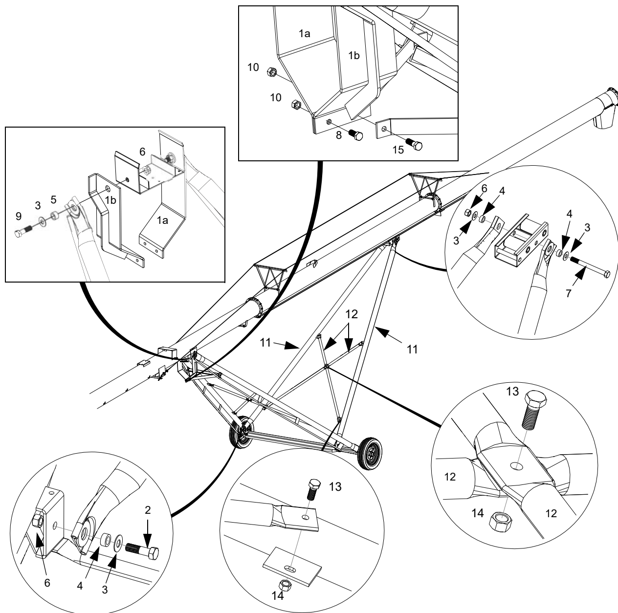
Figure 12. Connecting the Auger Tube to Frame
