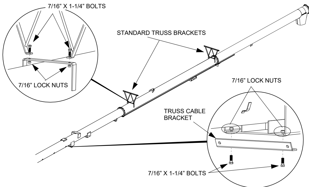
Figure 7. Truss Support and Truss Cable Brackets (64' Model)
