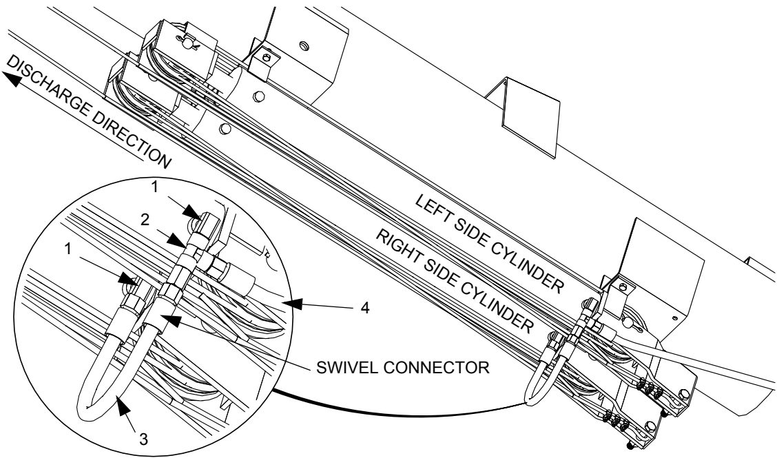
Figure 14. Hydraulic Fittings and Hoses
