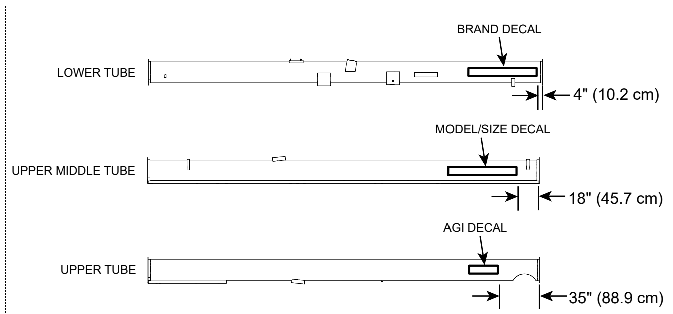
Figure 1. 64' Auger Tube Sections
