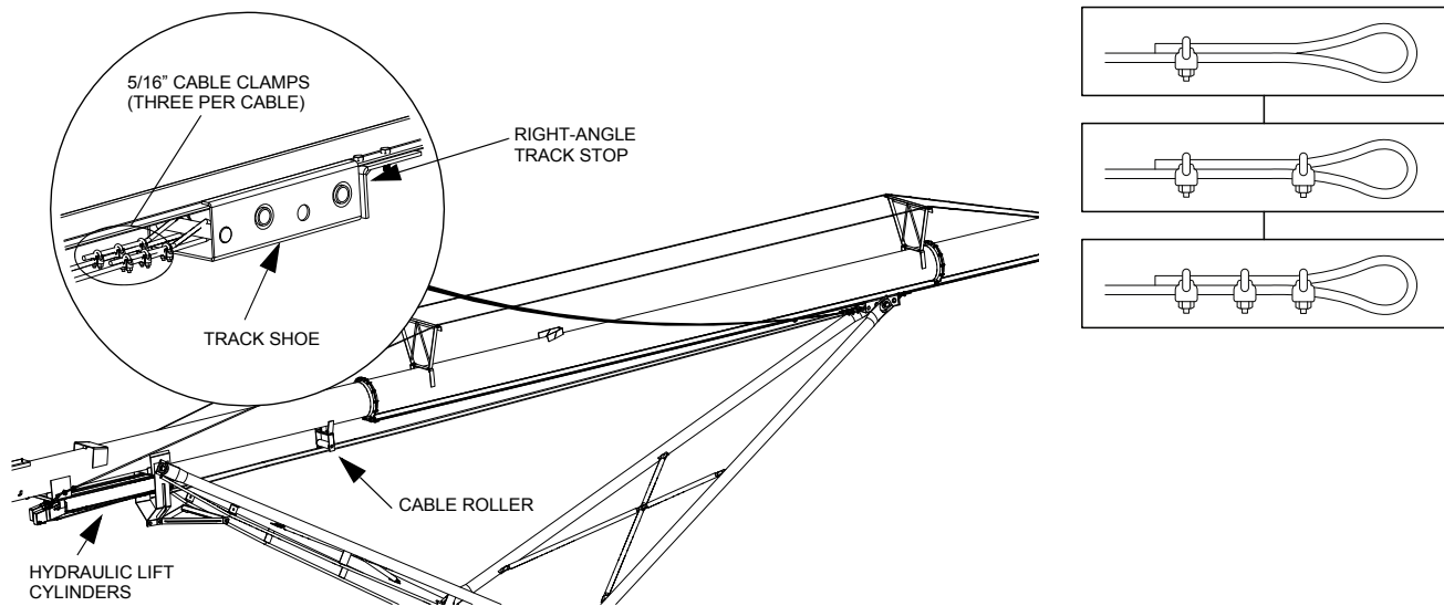
Figure 13. Connecting the Lift Cylinder Cables to the Track Shoe
