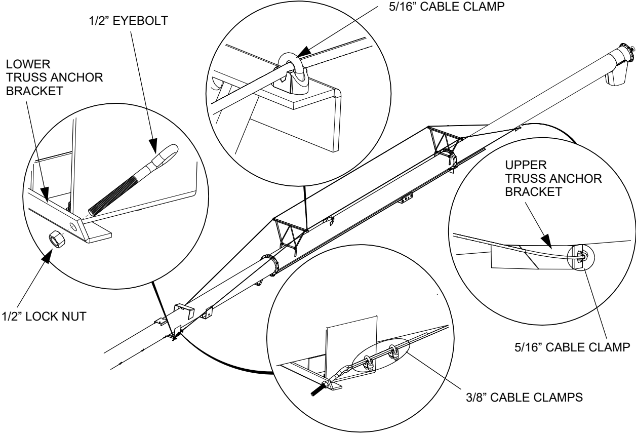
Figure 8. Truss Cables (64' Model)
