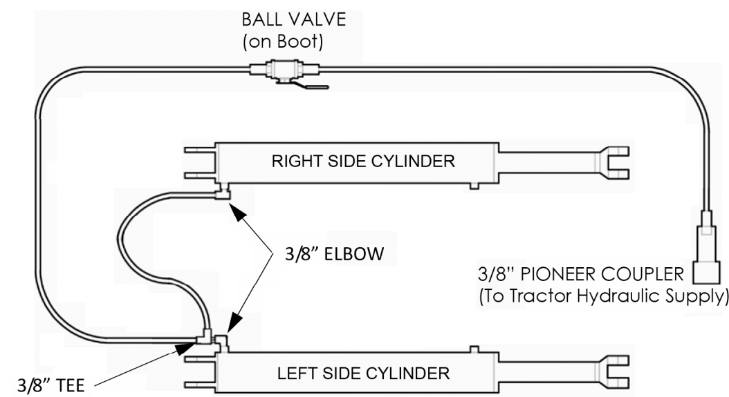
Figure 15. Hydraulic Diagram
