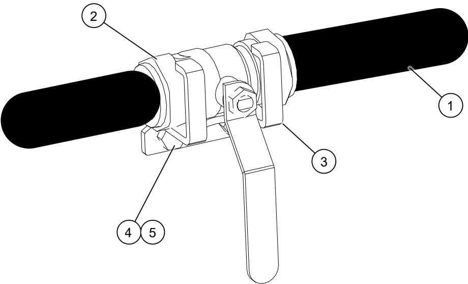
Figure 16. Installing the Ball Valve on the Boot
