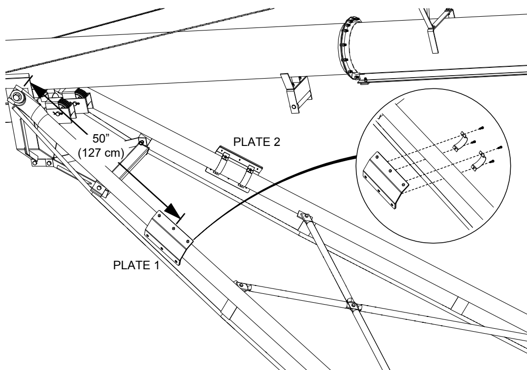
Figure 17. Installing the Frame Deflector Plates
