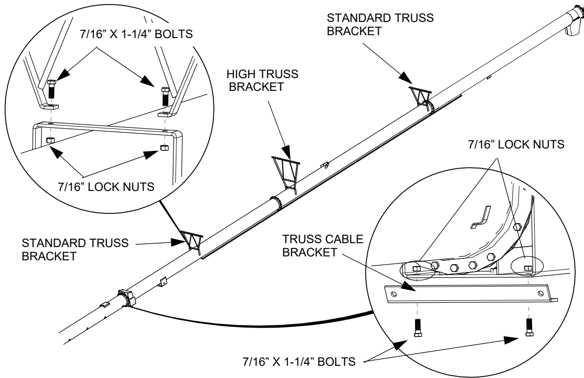
Figure 9. Truss Support and Truss Cable Brackets (74' Model)
