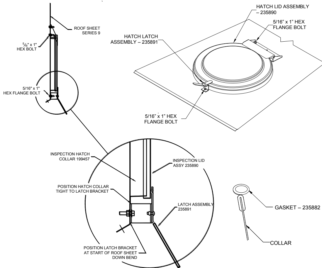
Figure 3. Inspection Hatch Details (9' - Optional)
