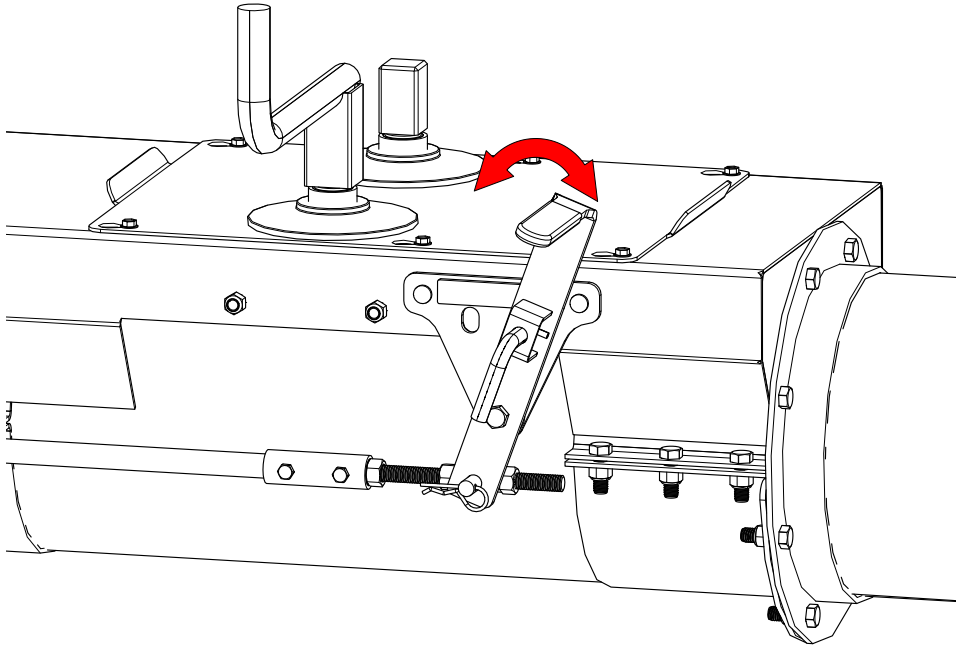
Figure 60. Lower Gearbox Engagement & Disengagement for Sweep
