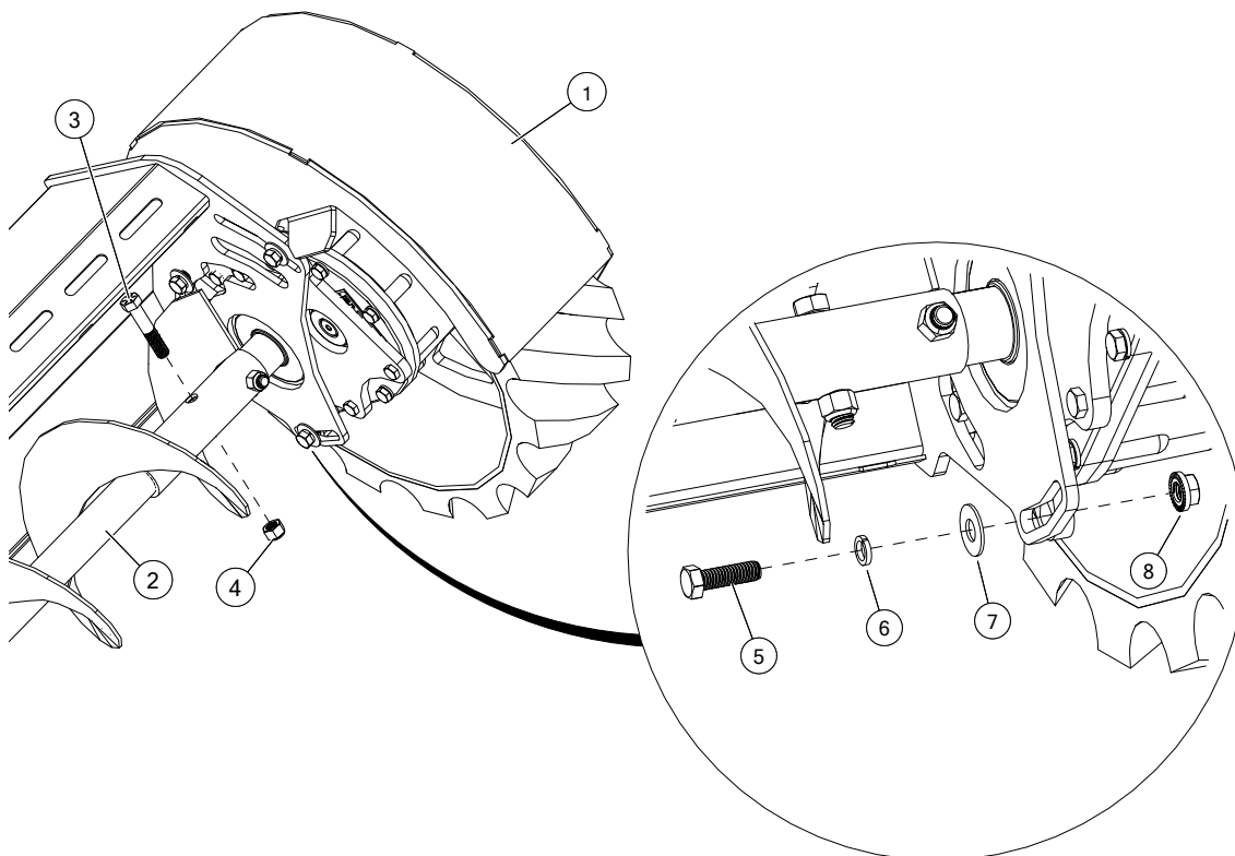
Figure 52. Install End Wheel Sub-Assembly
