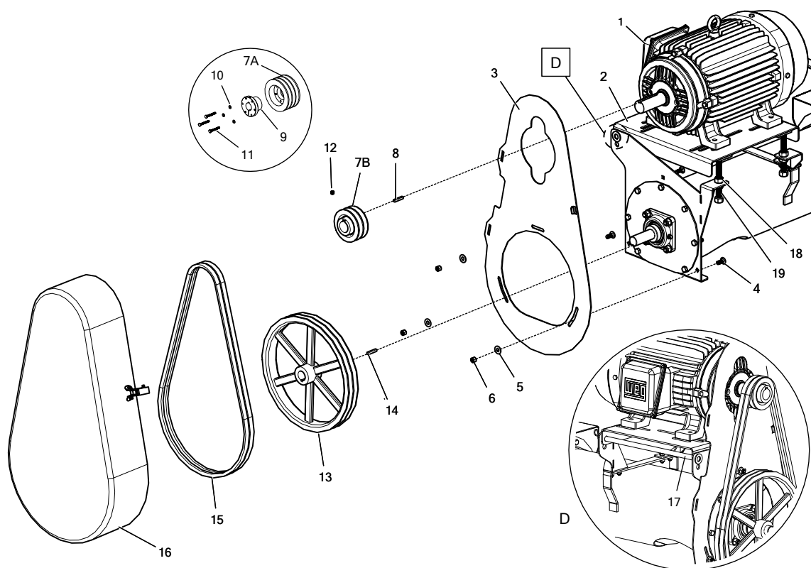
Figure 51. Assembly of Pulleys and Belts
