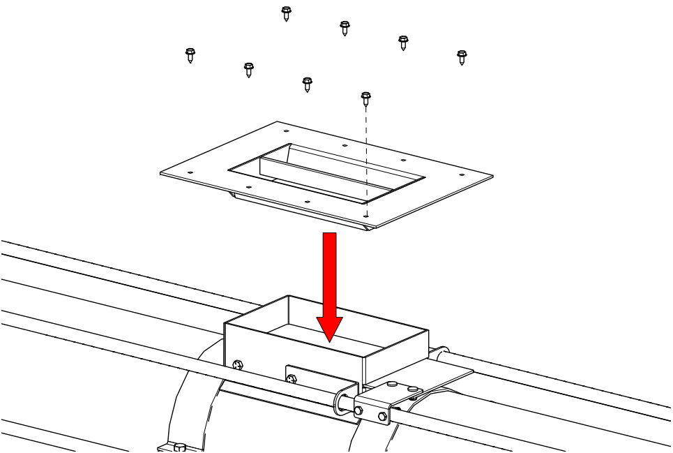
Figure 34. Install Grate(s) for Intermediate Sump(s) and E-Sump
