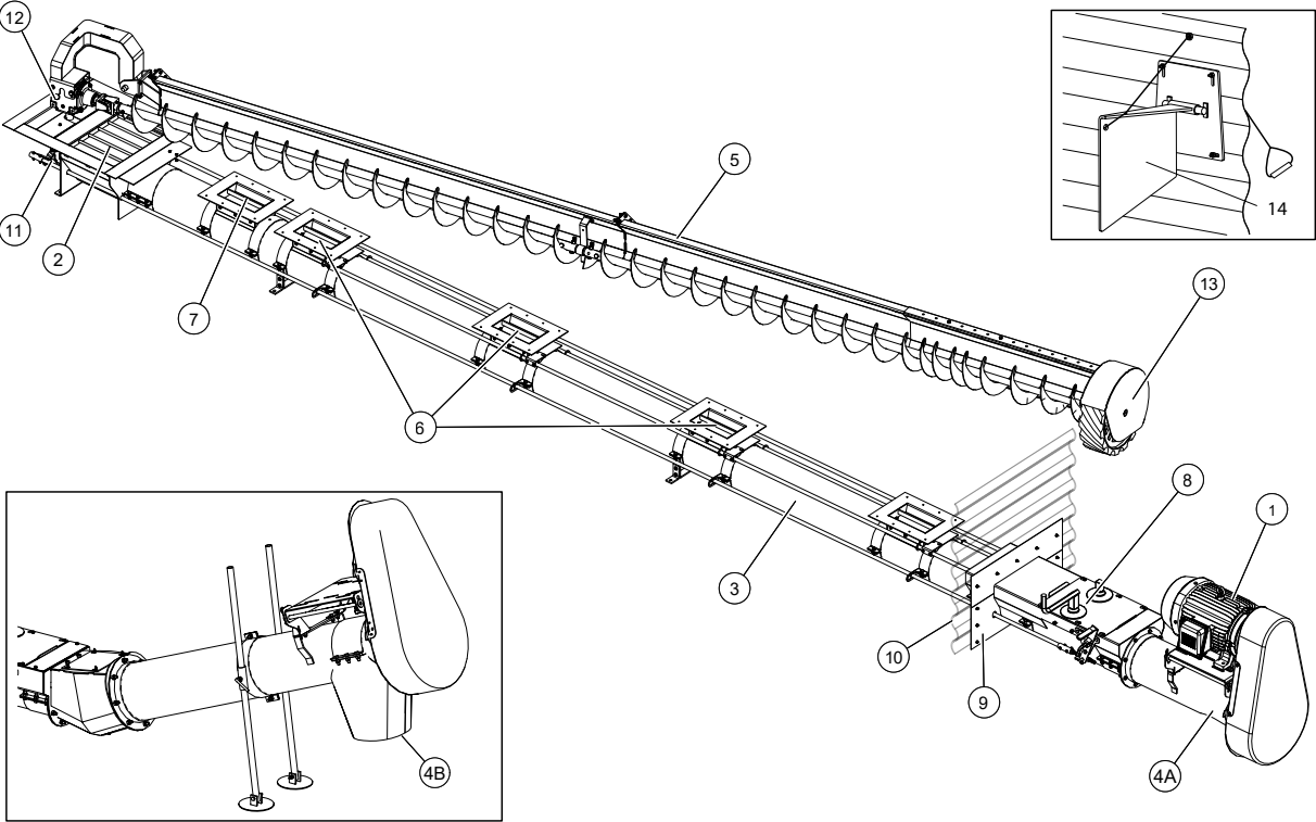
Figure 1. Typical Bin Unload System
