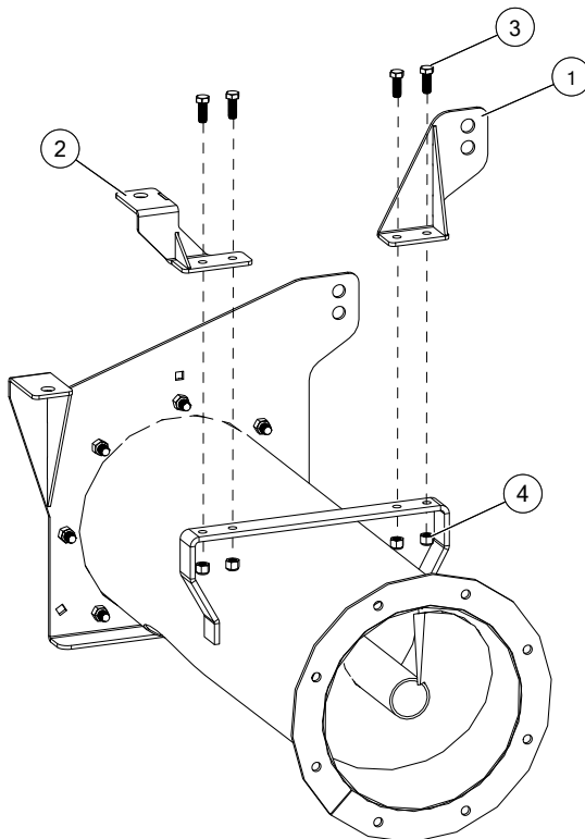
Figure 48. Rear Mount Plate and Support Bracket Installation
