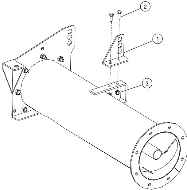
Figure 38. Rear Mount Plate and Support Bracket Installation
