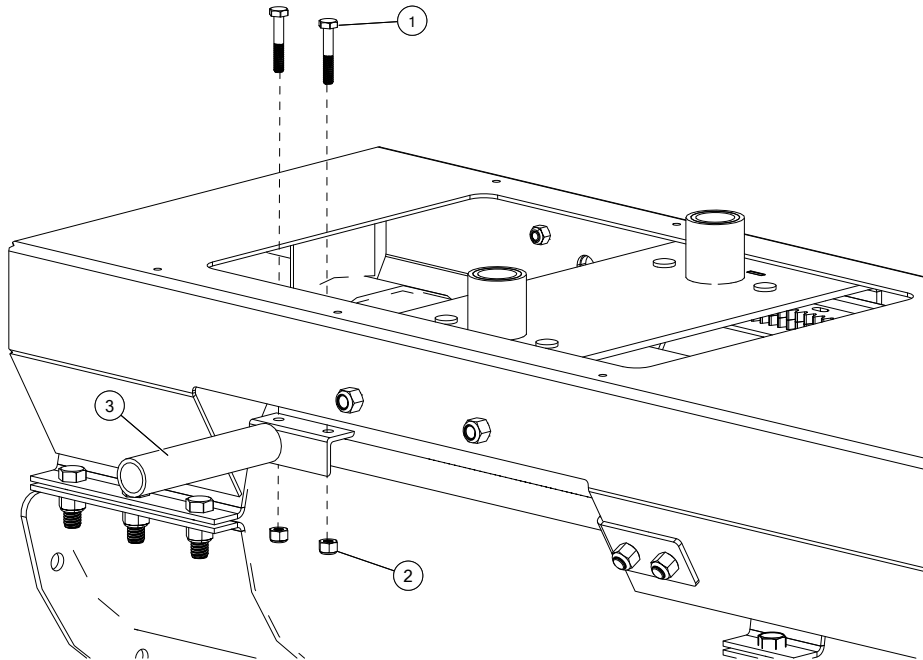
Figure 24. Install the E-Sump Control Handle
