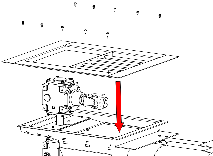
Figure 34. Install Grate(s) for Intermediate Sump(s) and E-Sump
