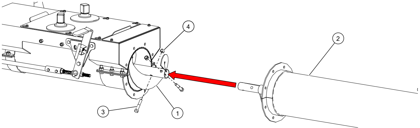
Figure 35. Fasten Extension Flighting onto Underfloor Auger Flighting
