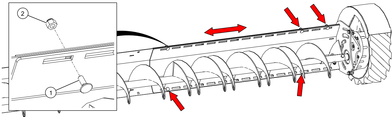
Figure 61. Adjust Bin Sweep Extension
