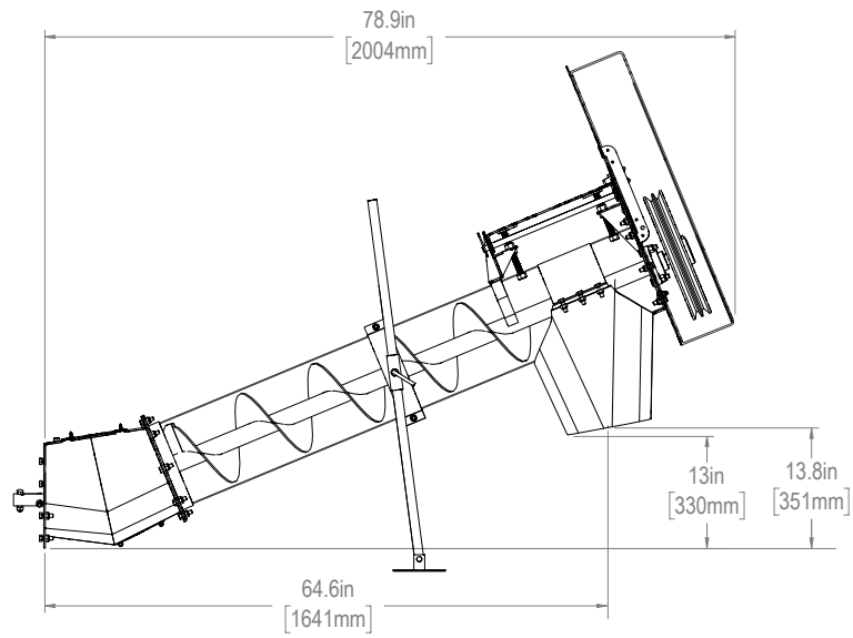
Figure 64. 8" Incline Tube Unload
