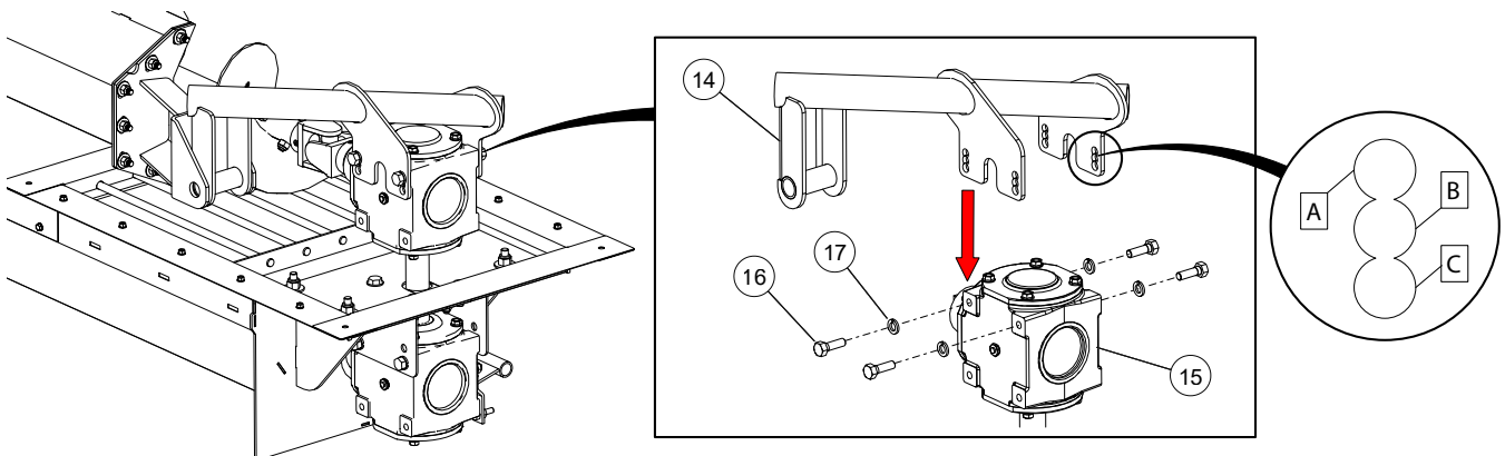
Figure 54. Attach Backboard Mounting Bracket on Upper Gearbox
