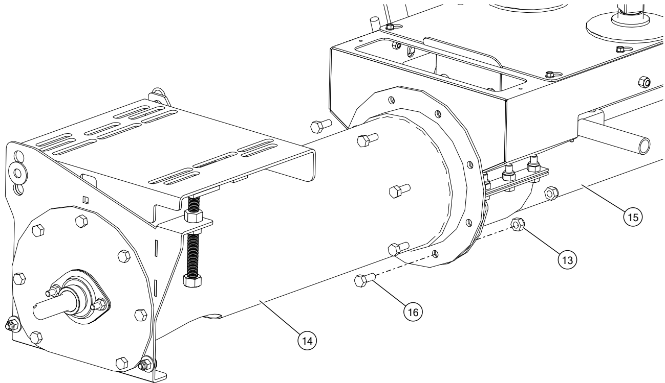
Figure 41. Mount Powerhead on the Underfloor Auger
