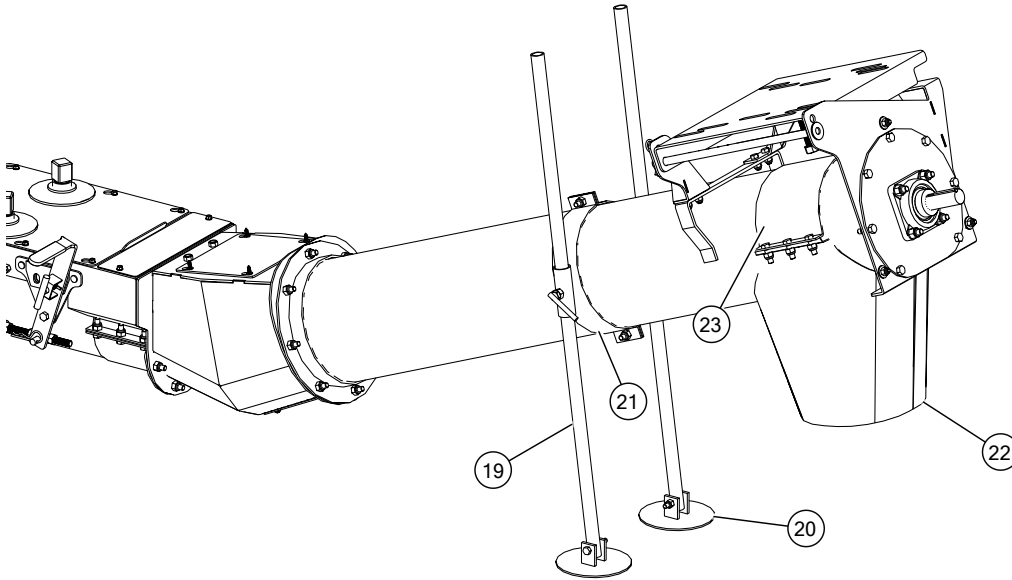
Figure 50. Assembled Incline
