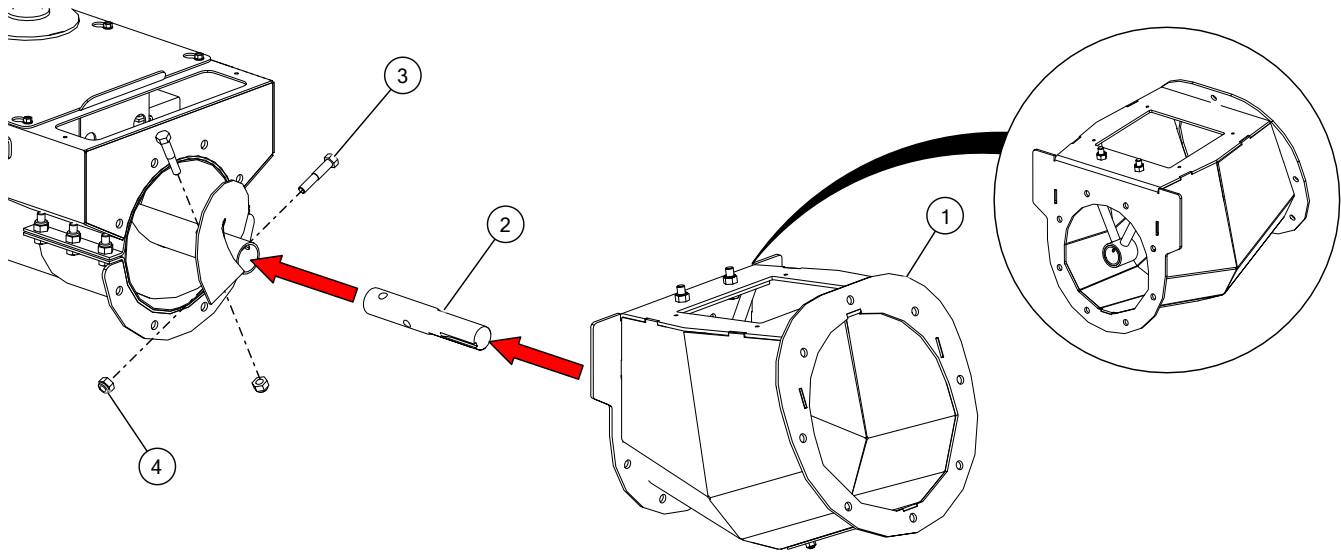
Figure 42. Installing the Transition Stub Shaft
