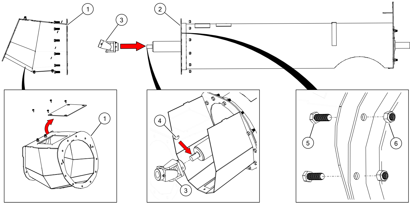
Figure 43. Attaching the Incline Transition to the Incline Powerhead
