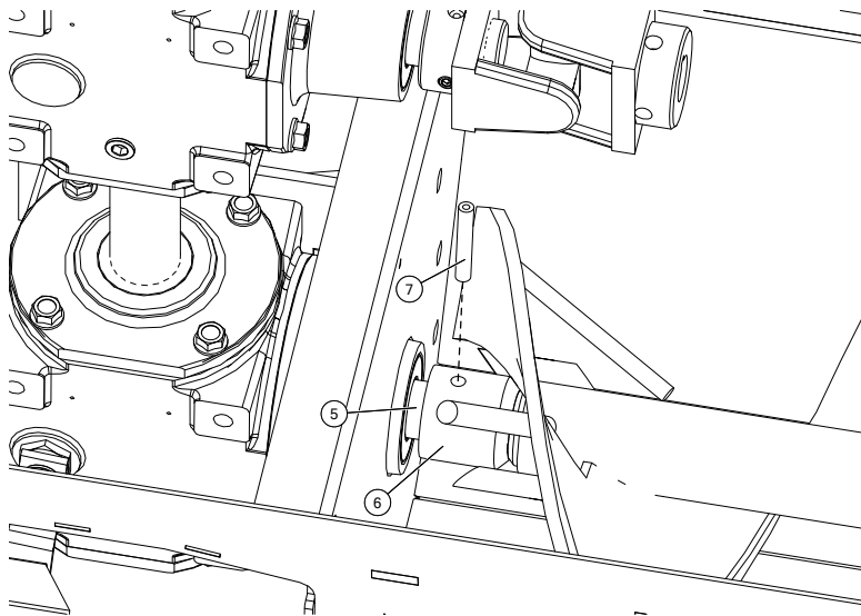
Figure 29. Attach Flighting to Lower Gearbox
