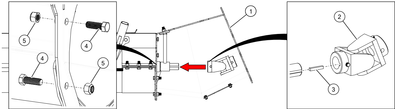
Figure 44. Connecting the Incline Assembly to Underfloor Auger
