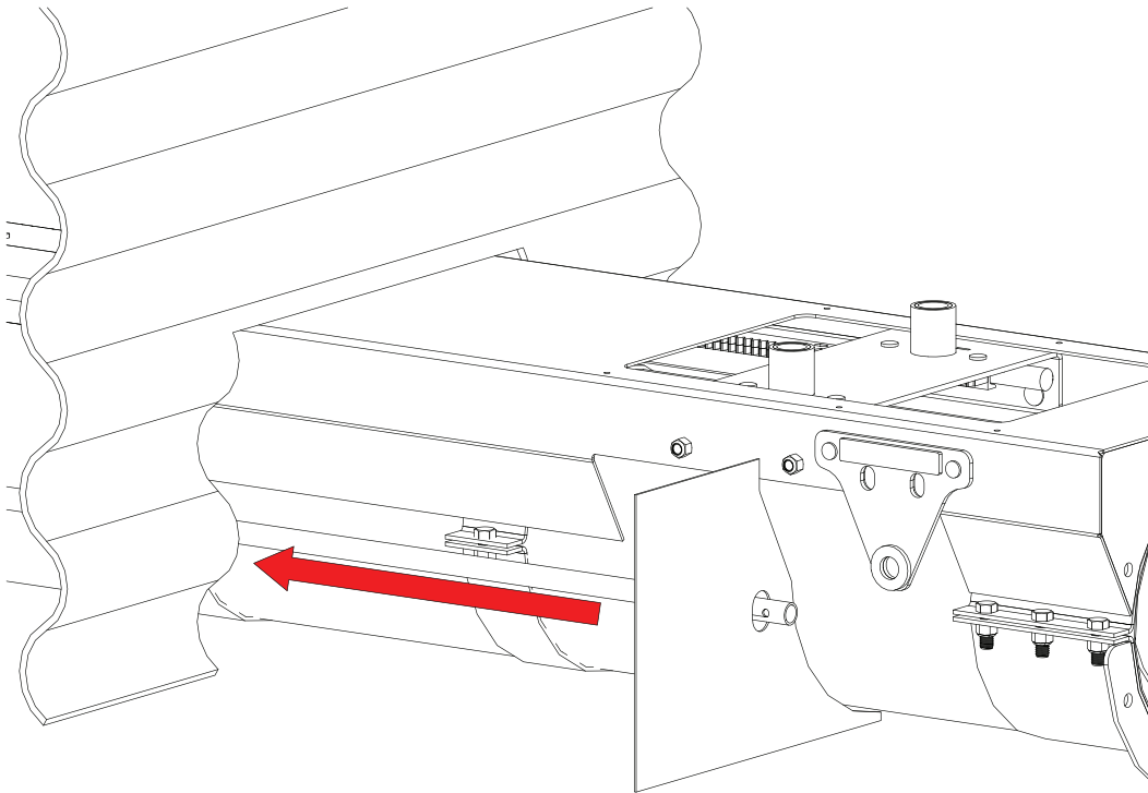
Figure 19. Slide Bin Adapter Piece on Lower Gearbox Control Rod
