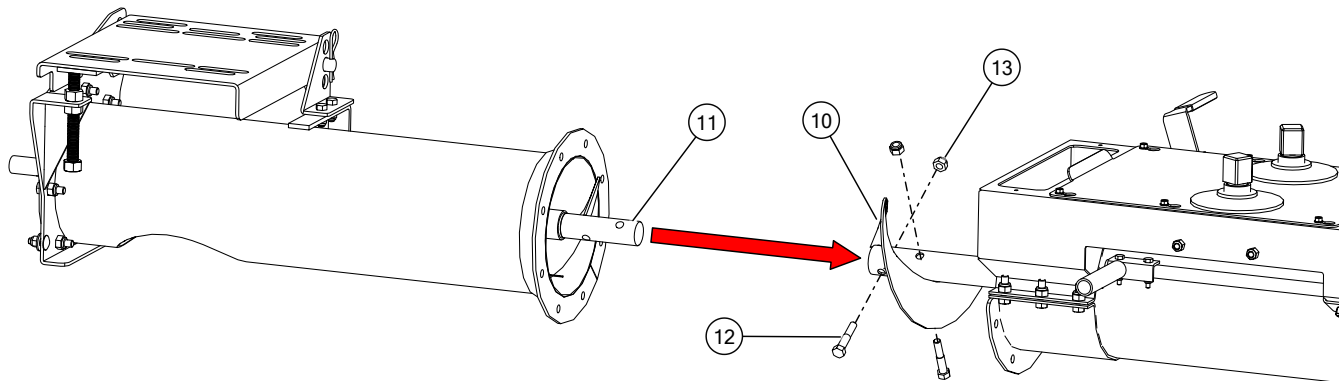
Figure 40. Fasten Discharge Flighting onto Underfloor Auger Flighting
