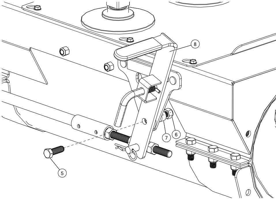
Figure 25. Connect the Gearbox Control Rod
