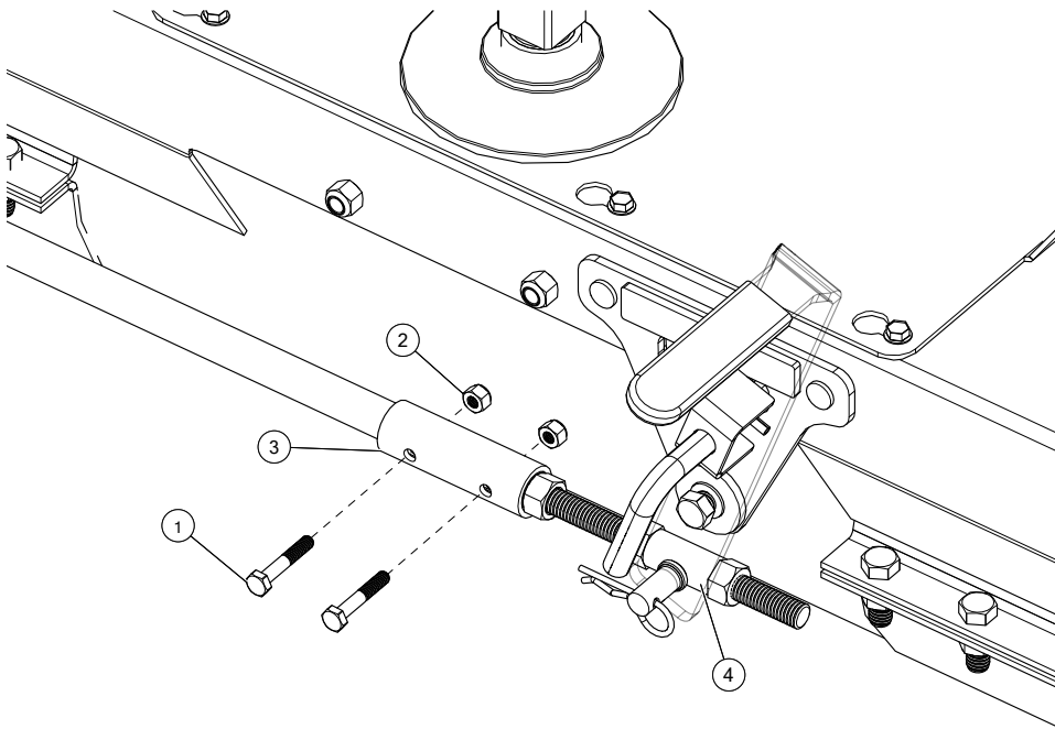
Figure 18. Unfasten the Coupler from the Gearbox Control Rod
