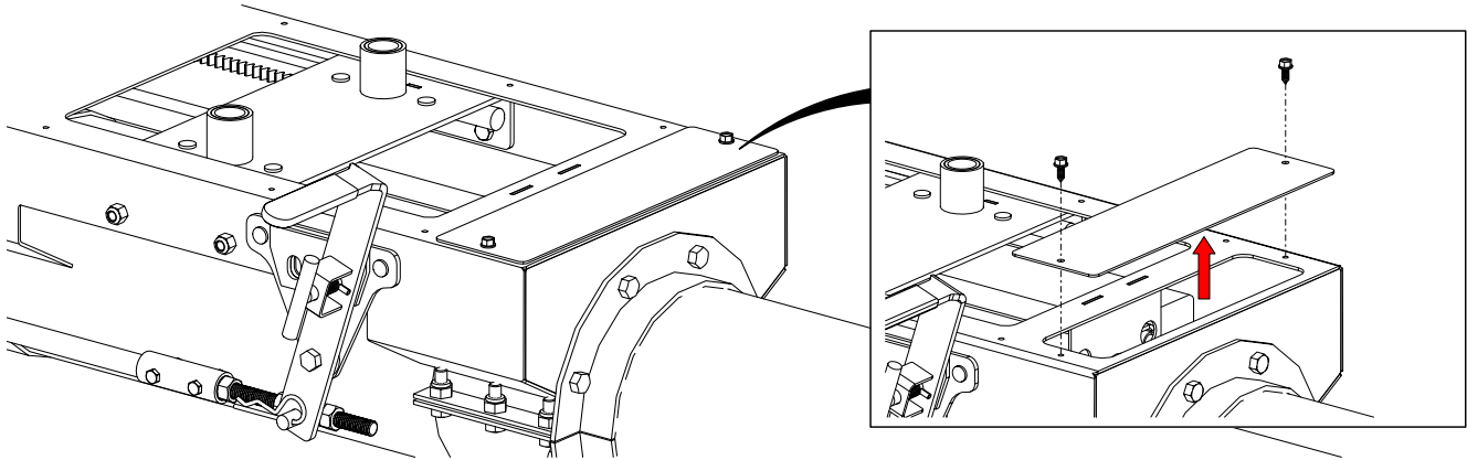
Figure 16. Remove Controls Cover
