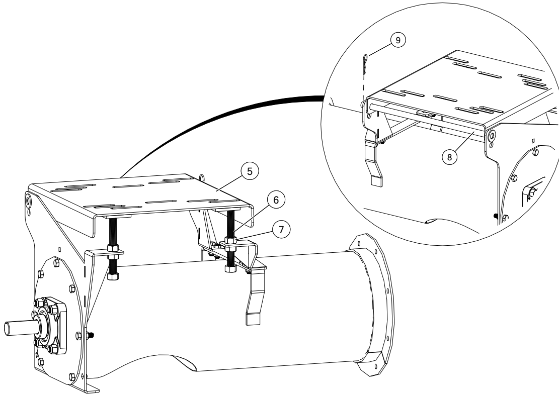
Figure 49. Install the Motor Mount Plate
