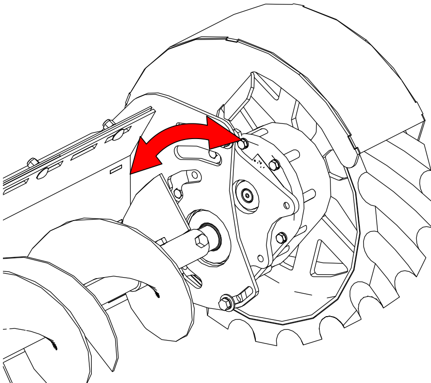
Figure 56. Adjusting Sweep Backboard Height at Sweep Drive Wheel
