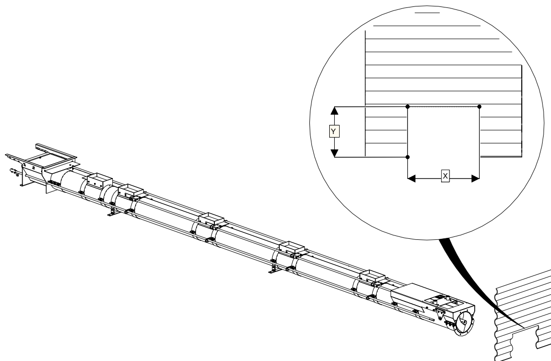
Figure 4. Bin Wall Cutout
