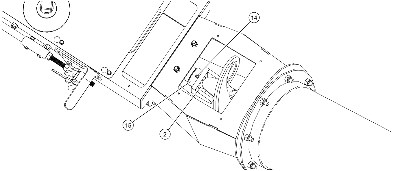
Figure 45. Secure Set Screws in Universal Joint for Transition Stub Shaft
