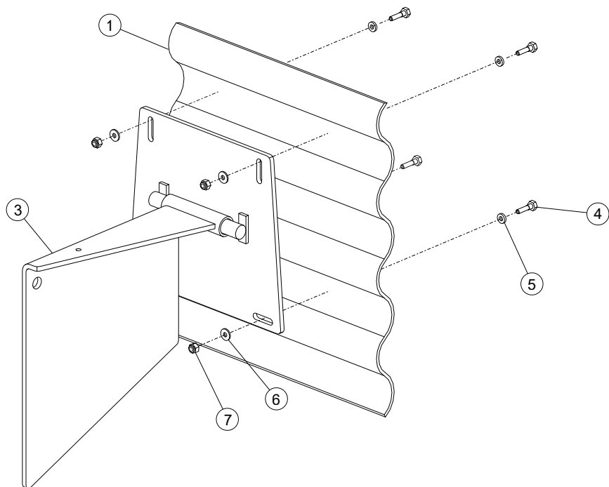
Figure 58. Install the Sweep Stop
