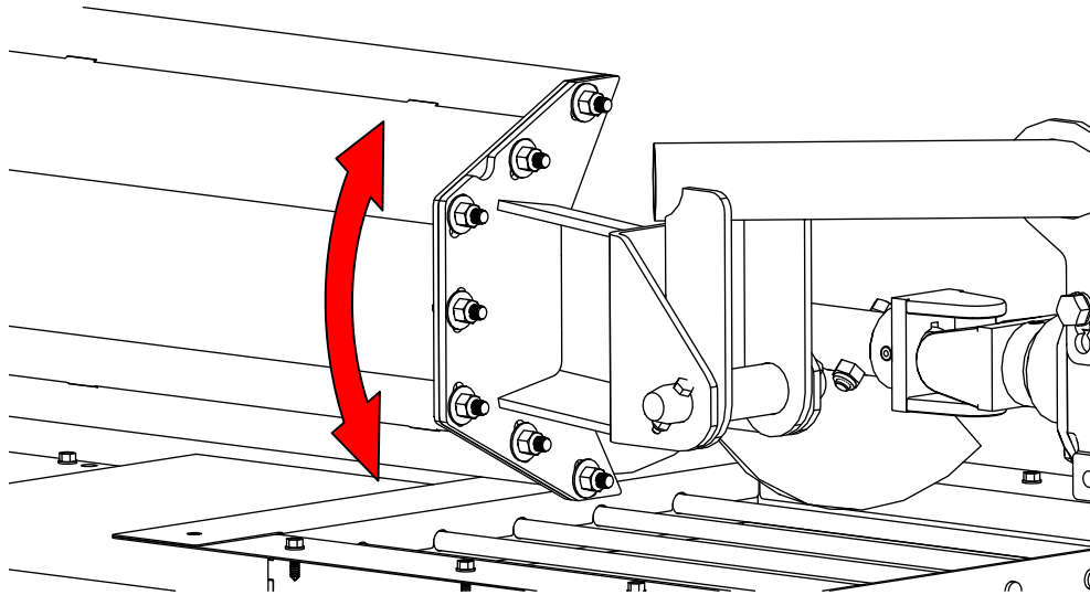
Figure 57. Adjusting Sweep Backboard Height Near Center Sump
