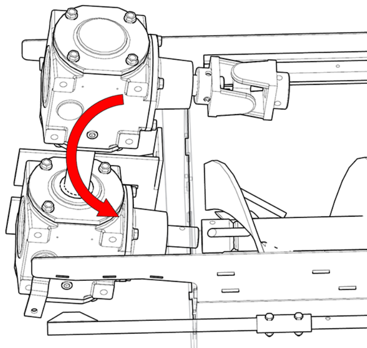
Figure 28. Install the Tandem Gearboxes
