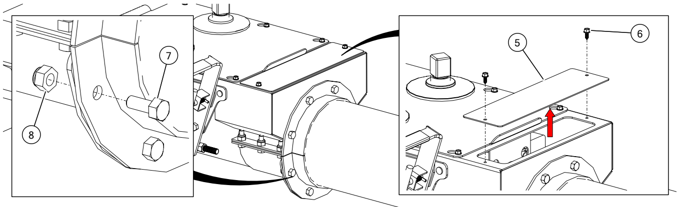
Figure 36. Mount Extension Tube onto Underfloor Flange
