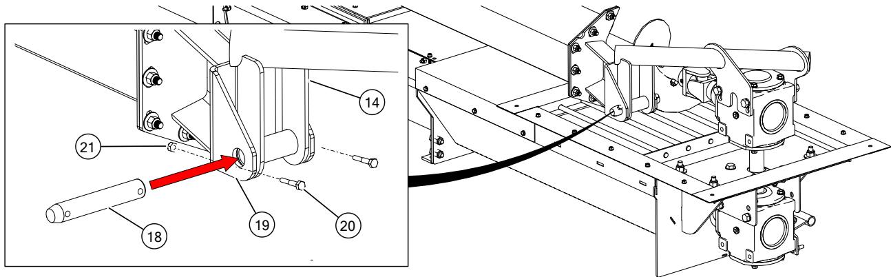
Figure 55. Connect Backboard Mounting Bracket to Backboard Connector
