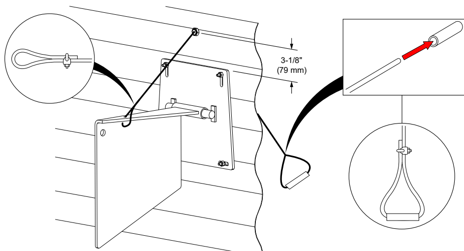
Figure 59. Route the Cable
