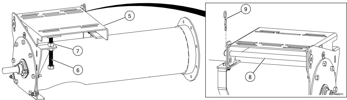
Figure 39. Install the Motor Mount Plate
