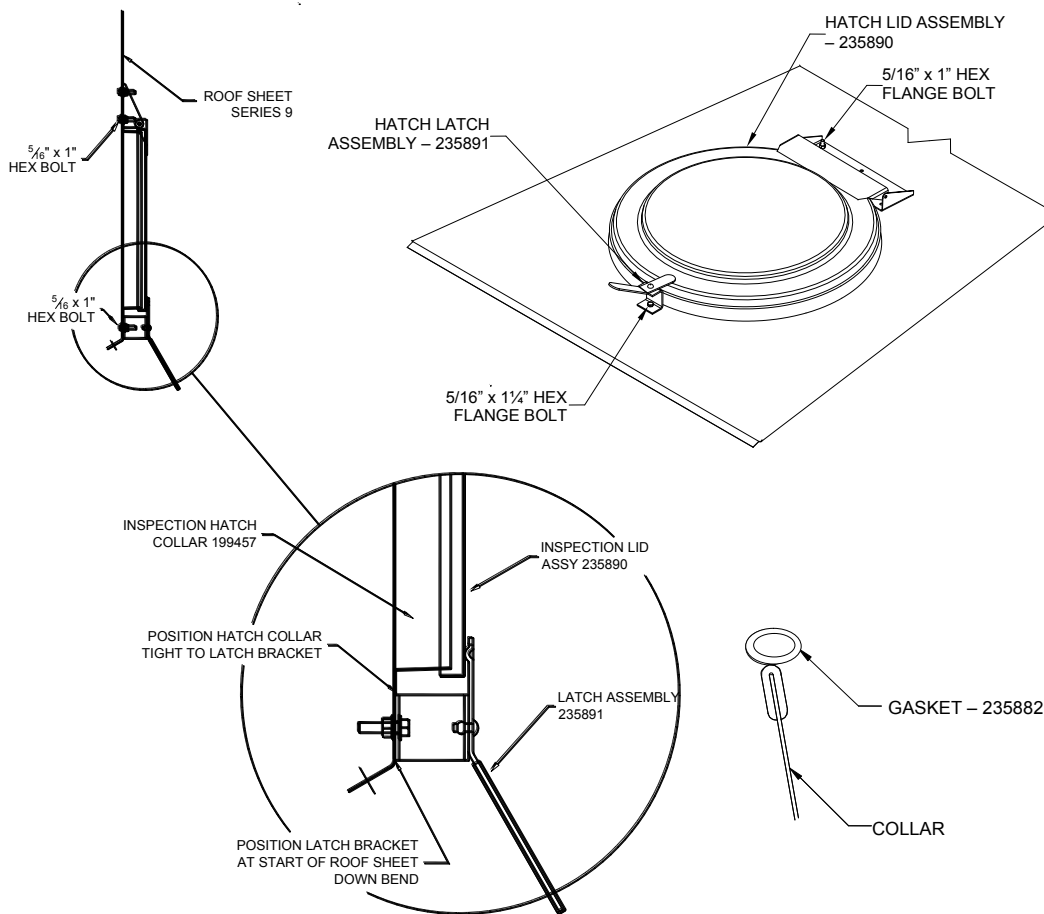
Figure 3. Inspection Hatch Details (9' - Optional)
