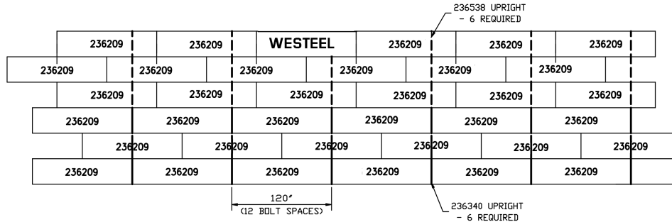
Figure 36. Model 196 — Cone Mount Bin (without door)
