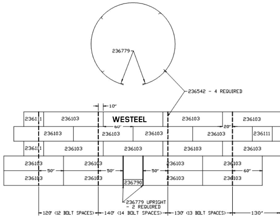
Figure 12. Model 145 — Door in second and third tiers
