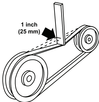
Figure 65. Typical Drive Belt Tensioning
