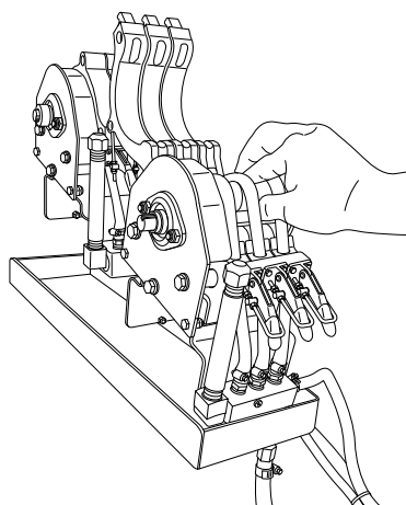
Figure 55. Chemical Pump Rollers
