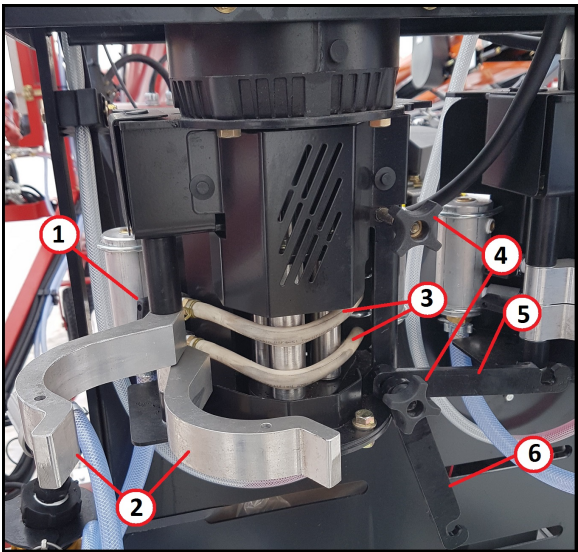
Figure 8. Pump Overview
