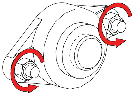
Figure 63. Loosen the Bearing Nuts
