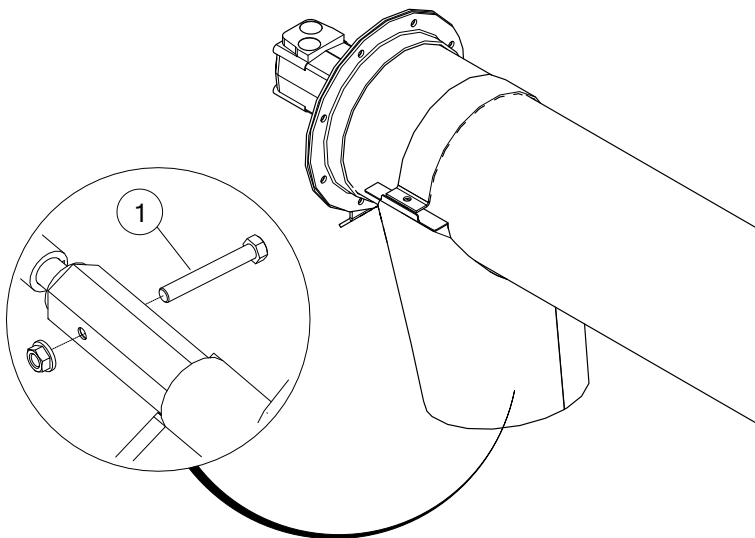
Figure 71. Removing the Shear Bolt
