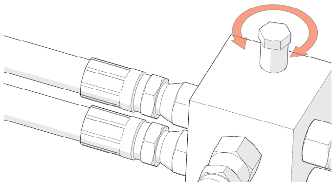
Figure 69. Cushion Valve Adjustment
