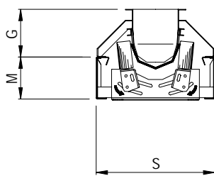
Inlet hopper section
