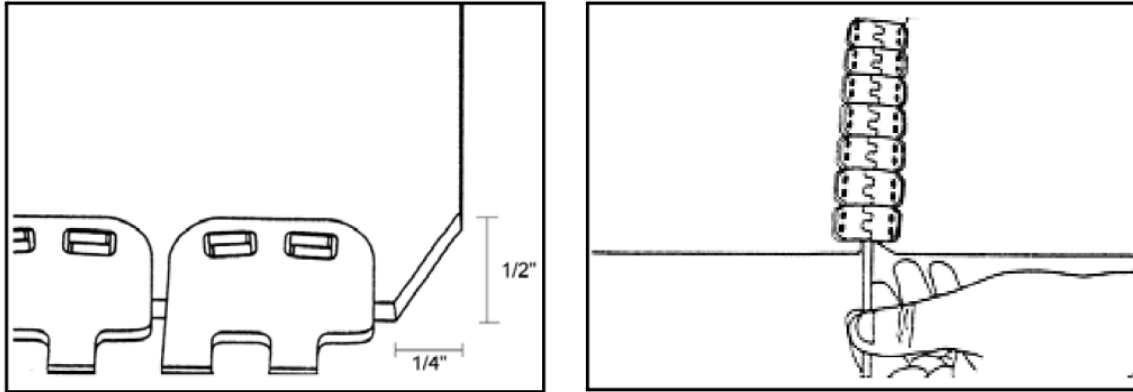
Figure 21. Lacing the Conveyor Belt
