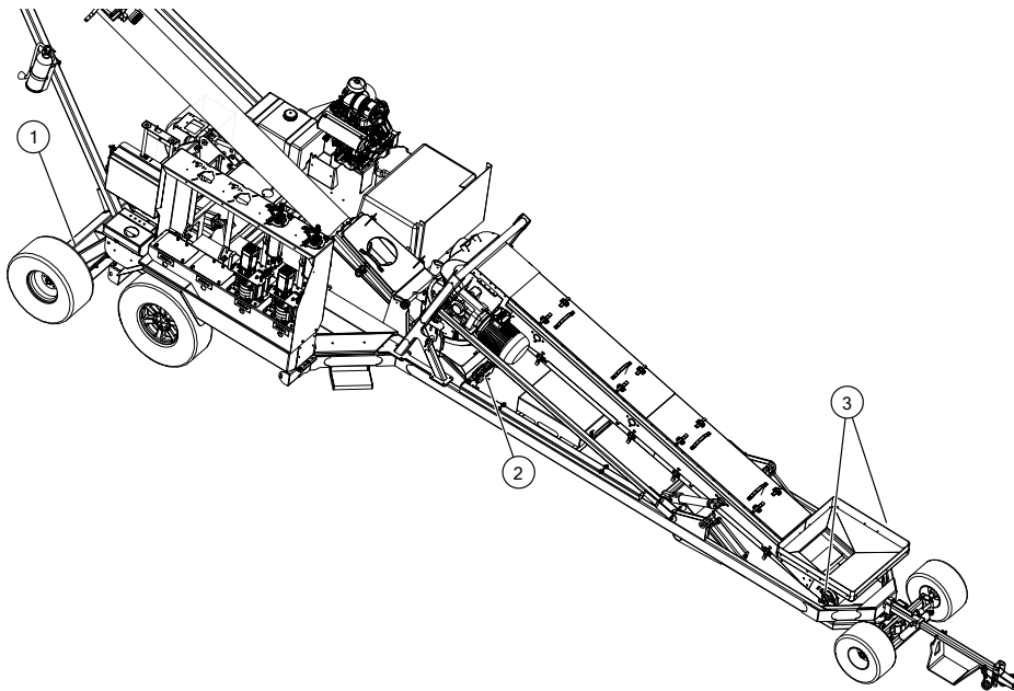
Figure 13. Bearing Locations
