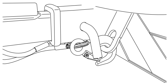
Figure 6. Correct Safety Cable Connection
