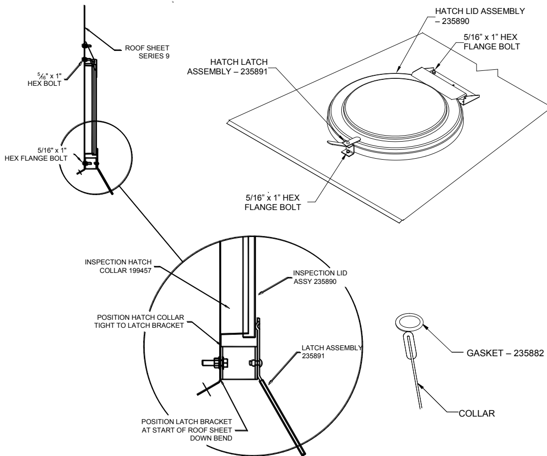
Figure 3. Inspection Hatch Details (9' - Optional)
