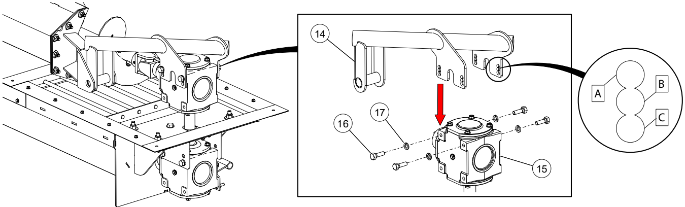
Figure 51. Attach Backboard Mounting Bracket on Upper Gearbox
