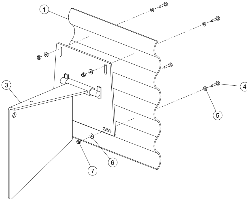
Figure 55. Install the Sweep Stop
