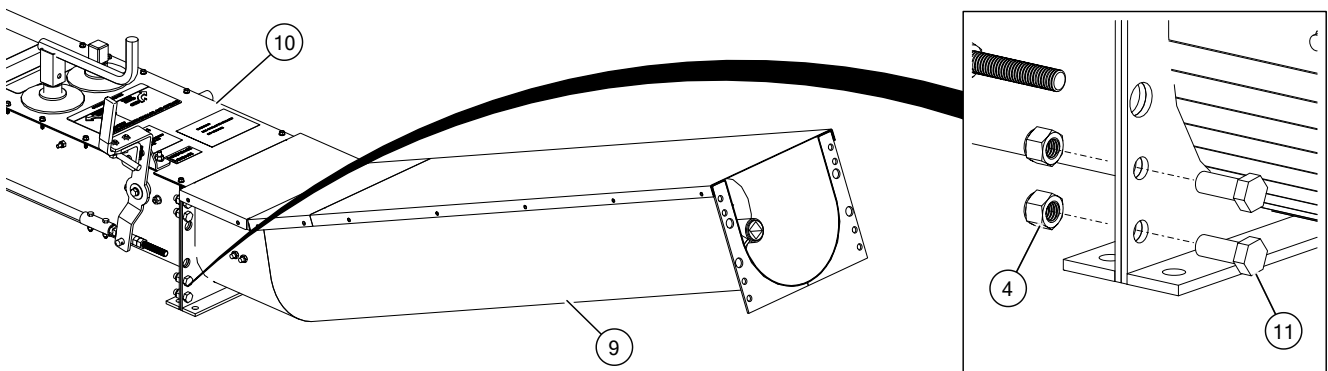
Figure 38. Fasten the Incline Assembly to the Underfloor Auger
