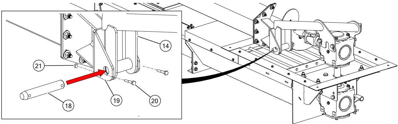
Figure 52. Connect Backboard Mounting Bracket to Backboard Connector
