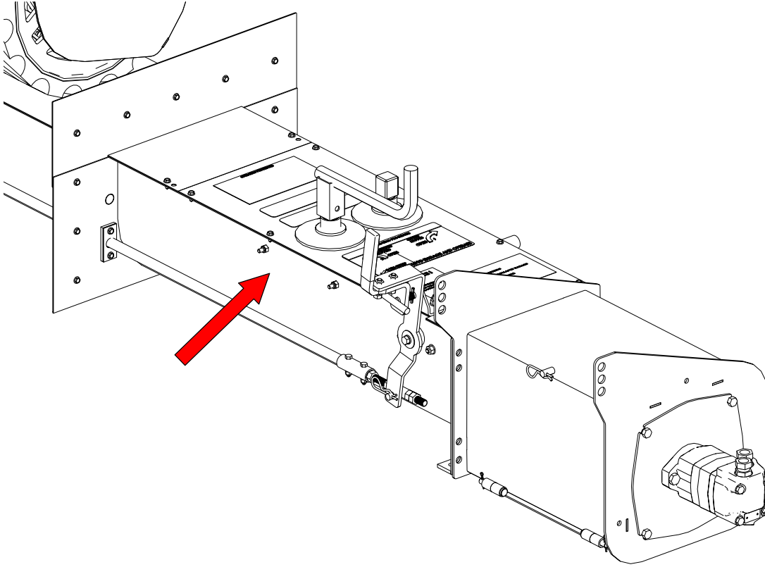
Figure 60. Placement for the Brand Logo Decal (Hydraulic Powerhead)
