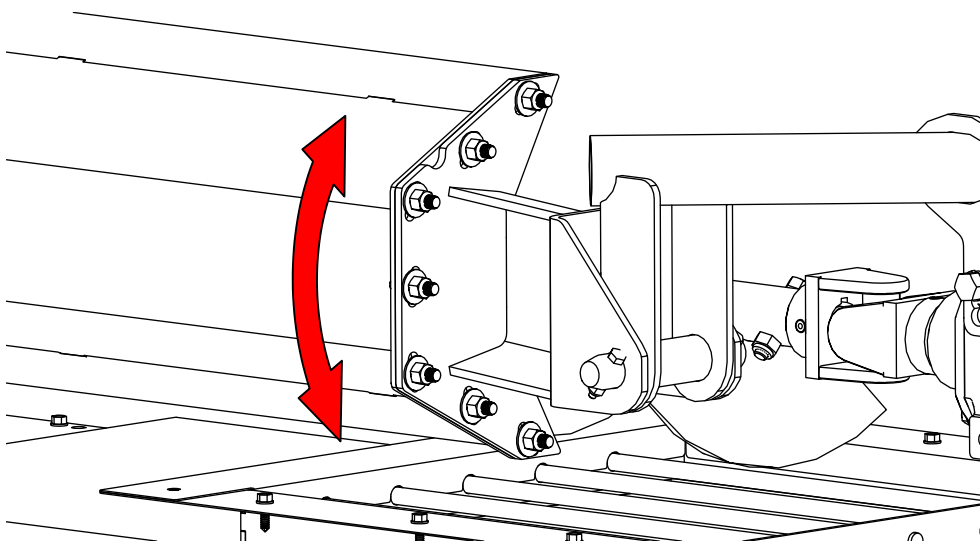
Figure 54. Adjusting Sweep Backboard Height near Center Sump
