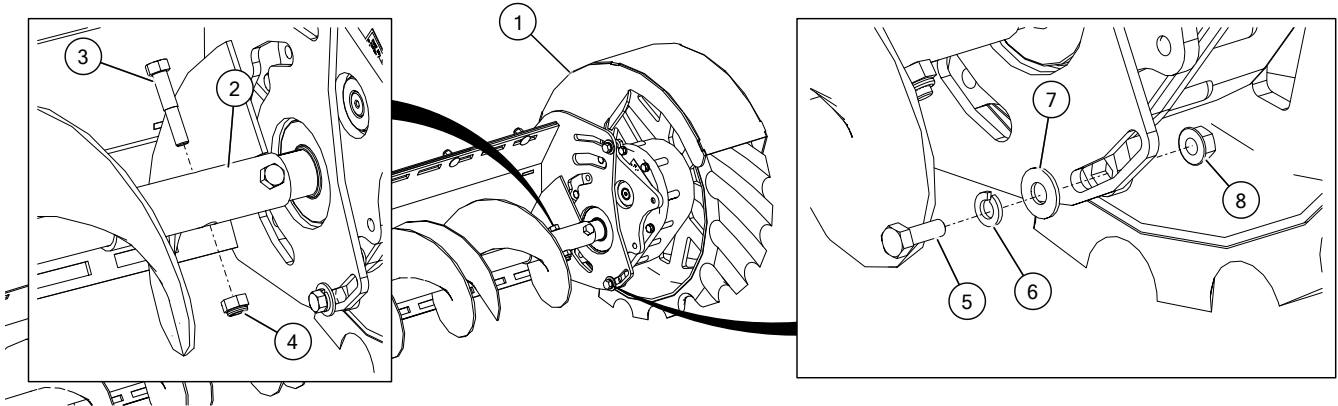
Figure 49. Install End Wheel Sub-Assembly
