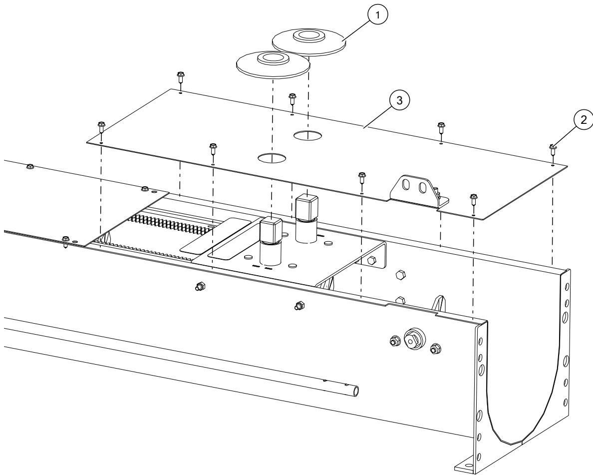
Figure 15. Control Cover Disassembly
