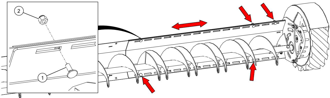
Figure 58. Adjust Bin Sweep Extension
