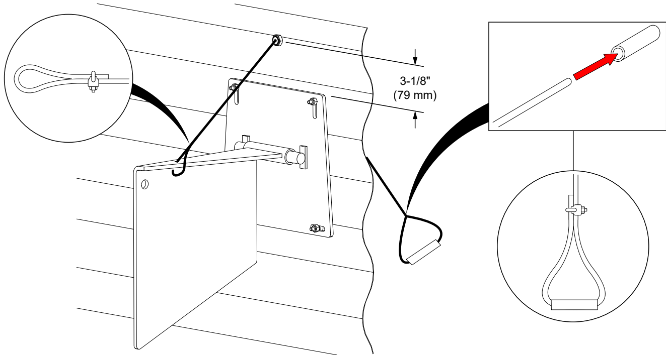
Figure 56. Route the Cable
