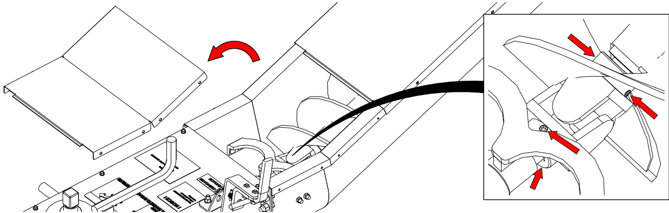
Figure 39. Secure Set Screws in Universal Joint
