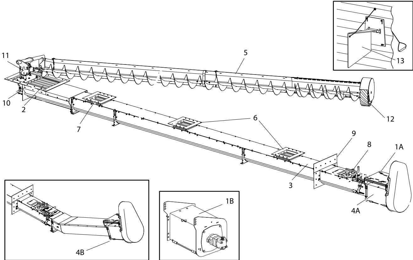
Figure 3. Bin Unload System Features
