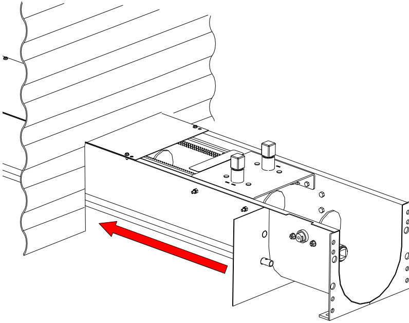
Figure 28. Slide Bin Adapter Piece on Lower Gearbox Control Rod
