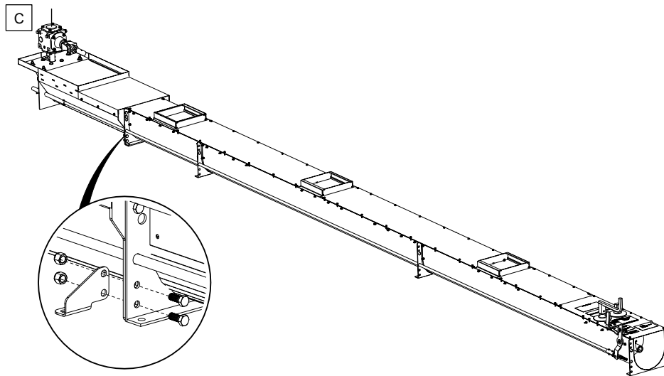
Figure 25. Install Underfloor Auger in Position
