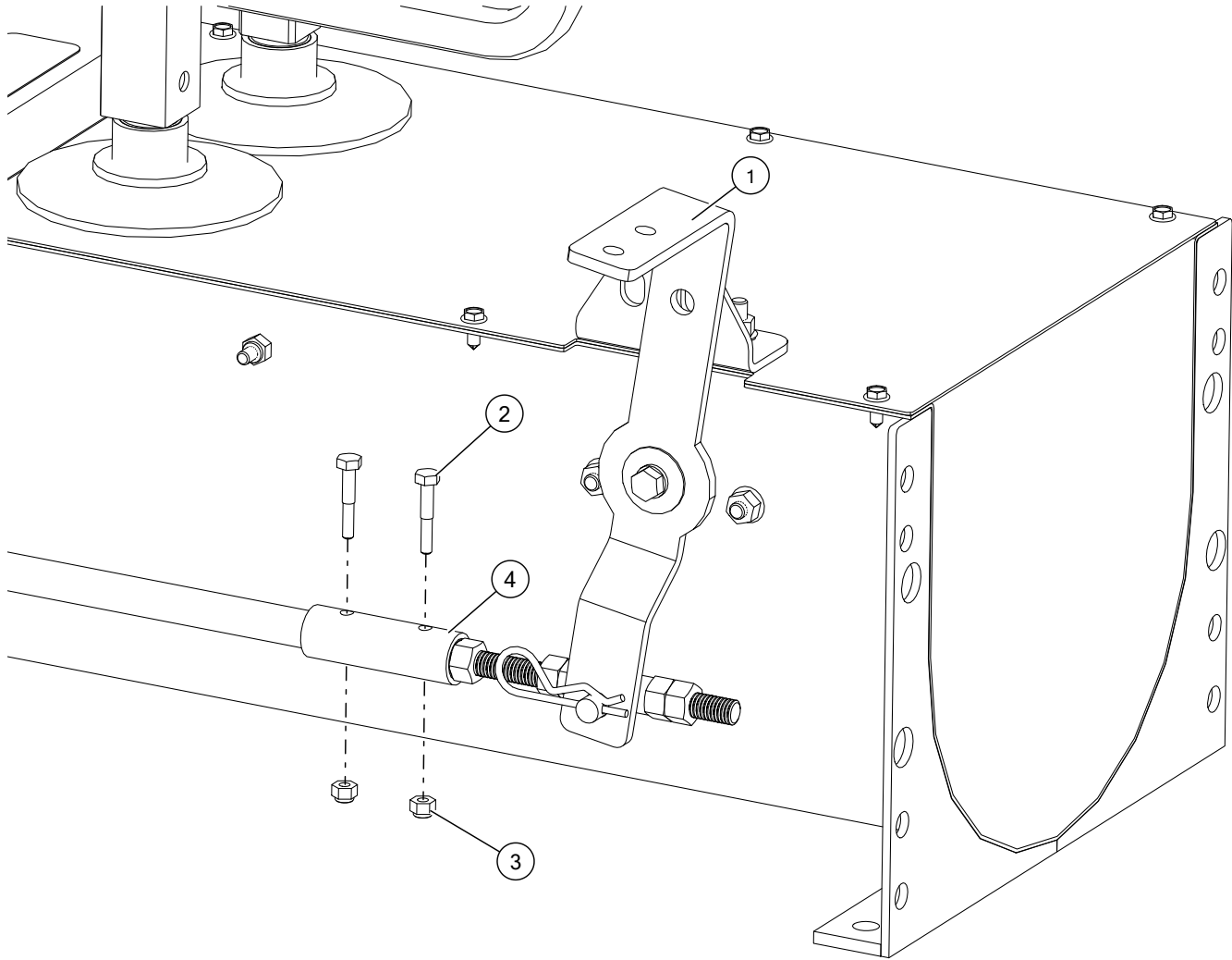
Figure 26. Unfasten the Coupler from the Gearbox Control Rod
