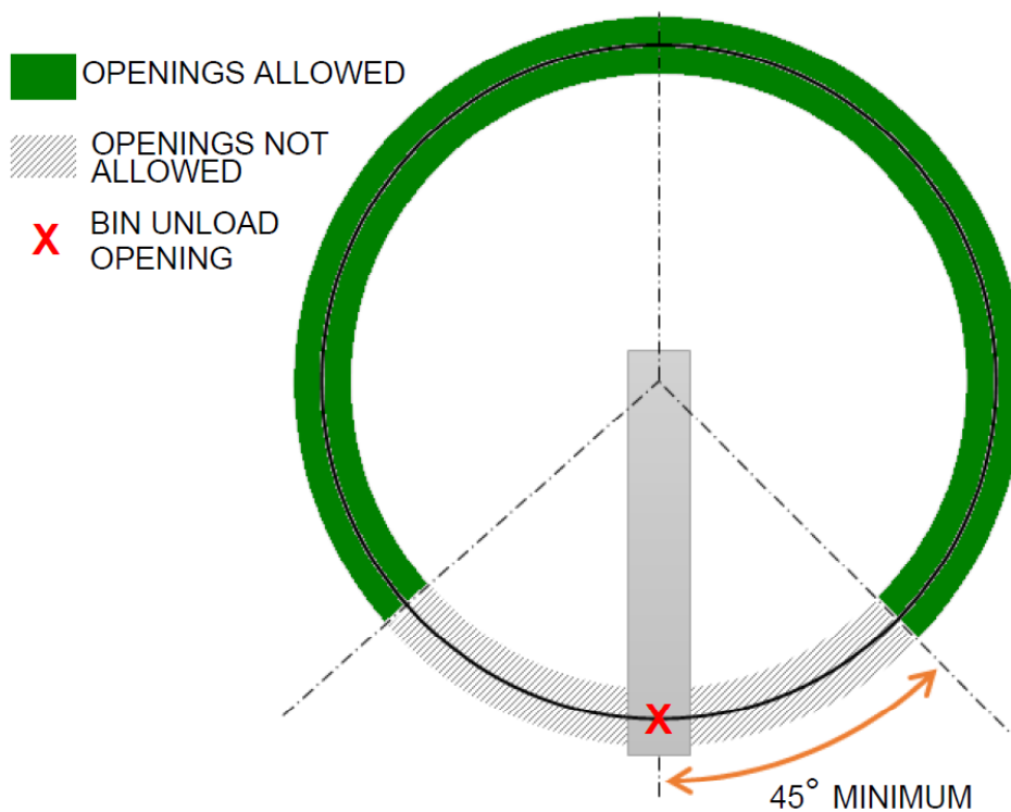
Figure 5. Minimum Angle Between Openings
