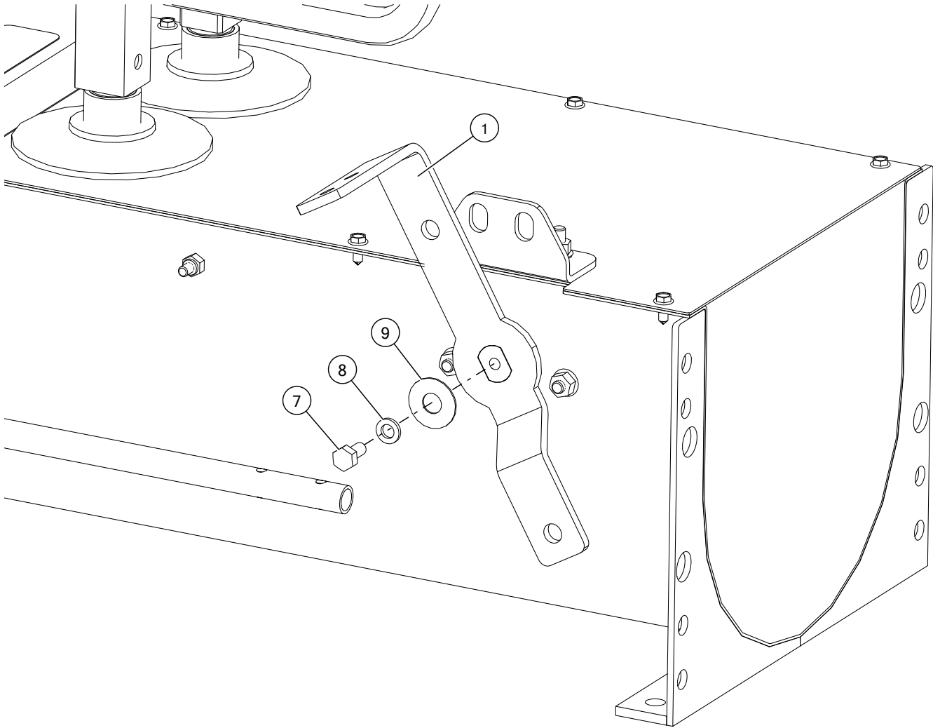
Figure 14. Remove the Gearbox Shift Lever
