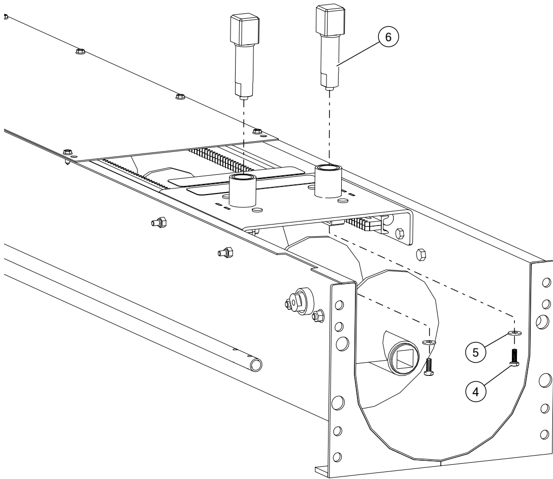
Figure 16. Remove the Sump Control Knob/Shafts
