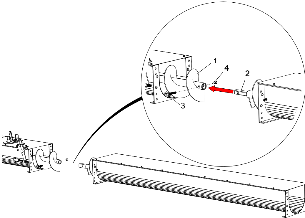
Figure 35. Fasten Extension Flighting onto Underfloor Auger Flighting
