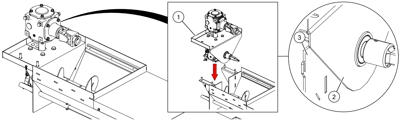
Figure 21. Lower the Gearbox into the Trough
