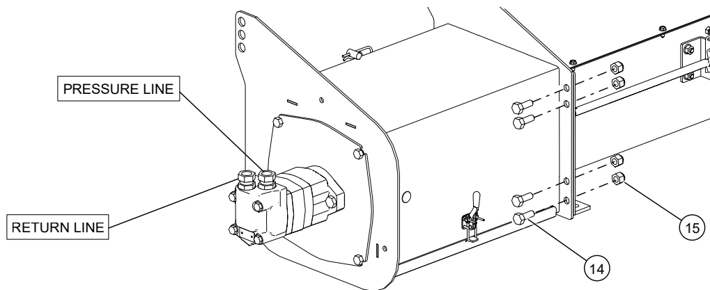
Figure 48. Mount Powerhead to Underfloor Auger
