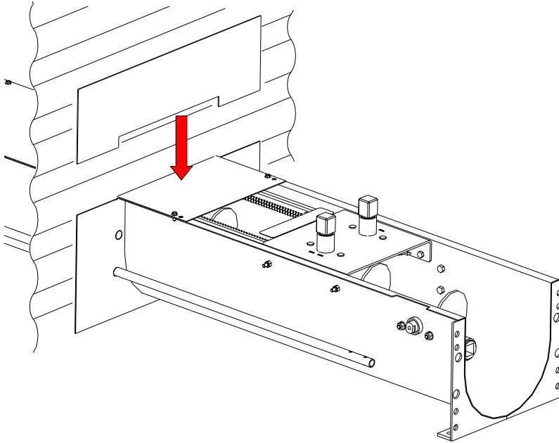
Figure 30. Position Bin Adapter Top Piece
