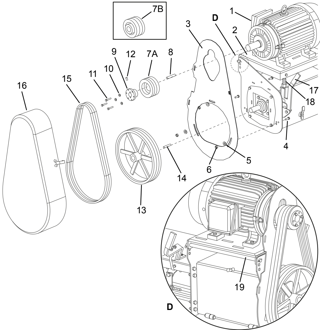
Figure 45. Assembly of Pulleys and Belts
