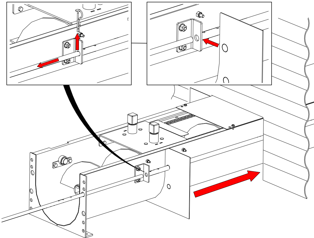
Figure 29. Slide Bin Adapter Piece
