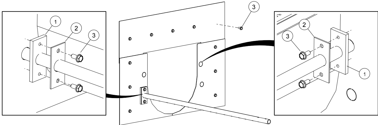
Figure 32. Screwing Bin Adapter Pieces
