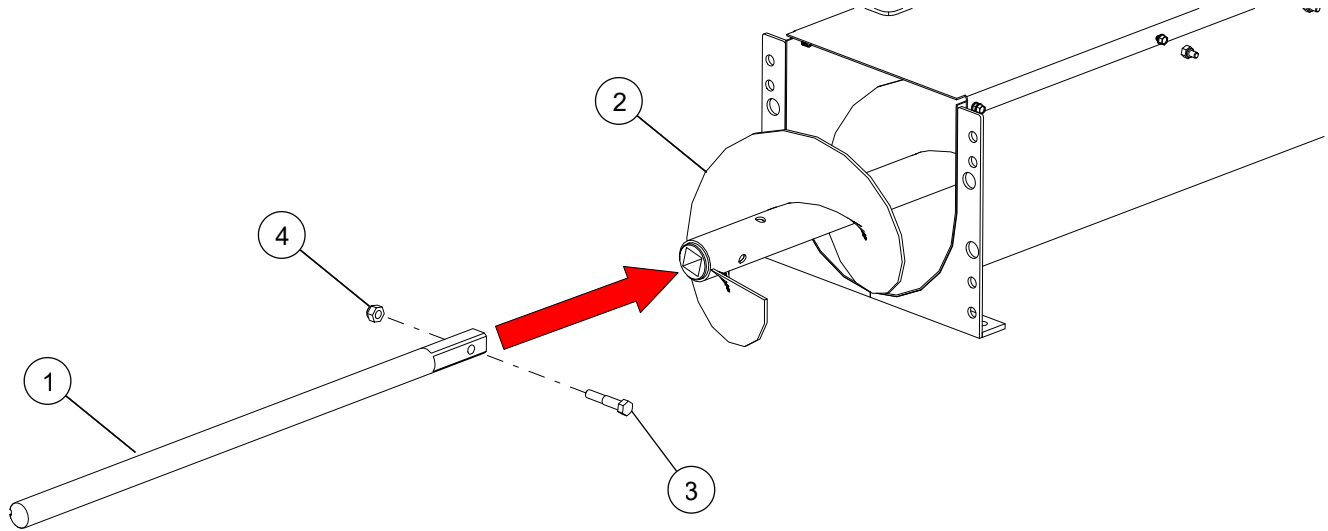
Figure 41. Fasten Shaft onto Underfloor Auger Flighting
