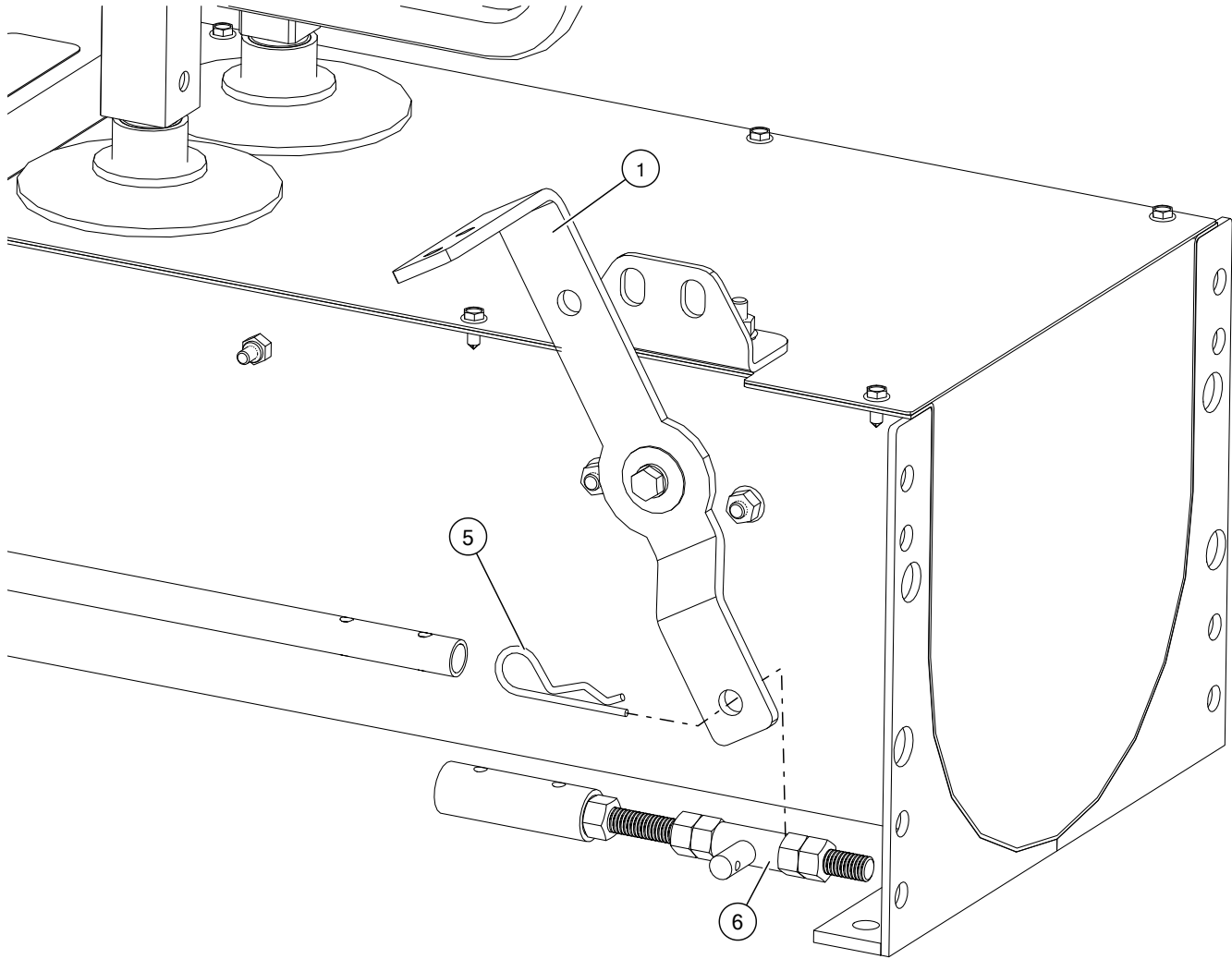
Figure 13. Remove the Coupler Assembly from the Gearbox Shift Lever
