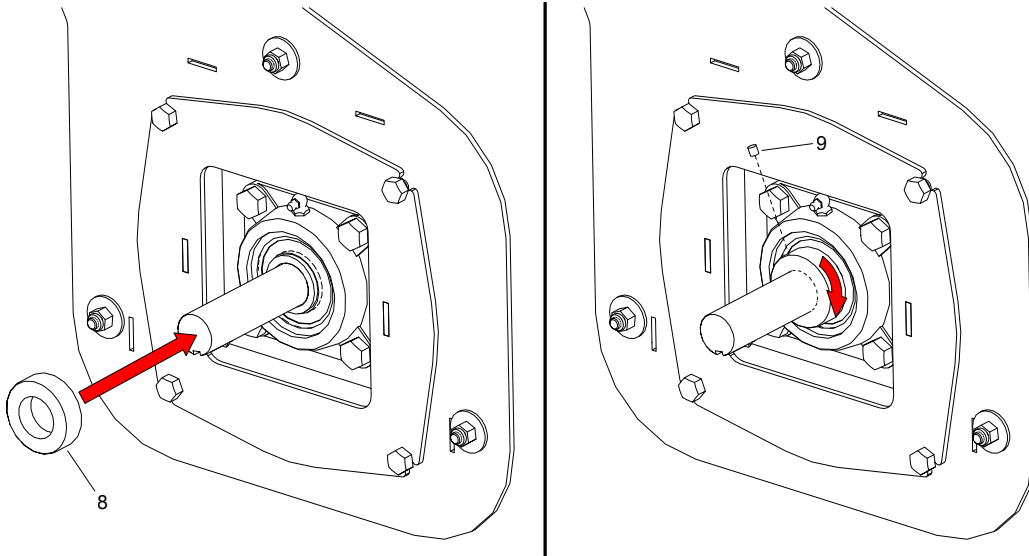
Figure 43. Mount the Bearing Lock Collar
