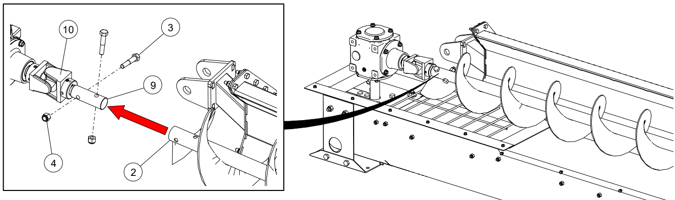
Figure 50. Connect Sweep Flighting to Upper Gearbox
