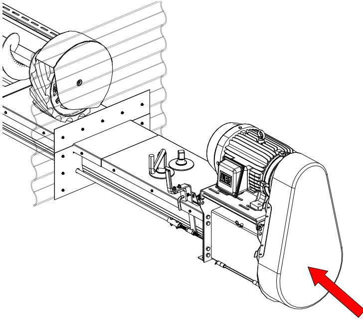
Figure 59. Placement for the Brand Logo Decal (Electric Powerhead)
