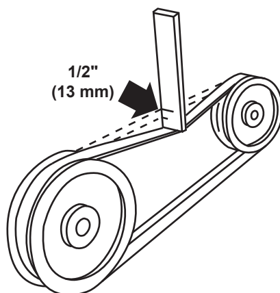
Figure 44. Typical Drive Belt Tensioning
