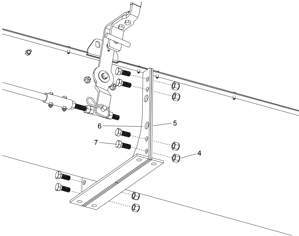
Figure 36. Mount Extension Trough onto Underfloor Flange
