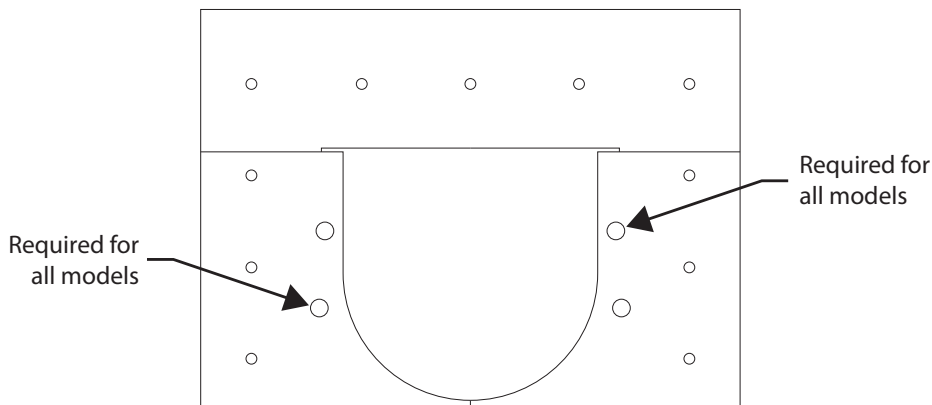
Figure 27. Control Rod Holes in Bin Adapter Piece
