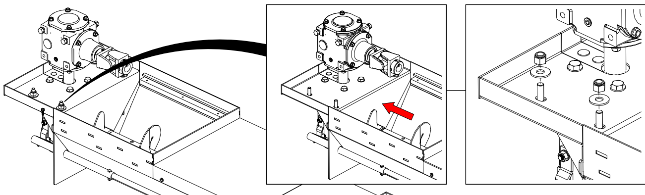
Figure 23. Install Tandem Gearboxes into Center Sump
