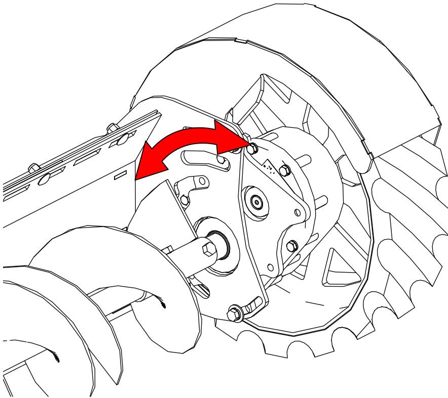
Figure 53. Adjusting Sweep Backboard Height at Sweep Drive Wheel
