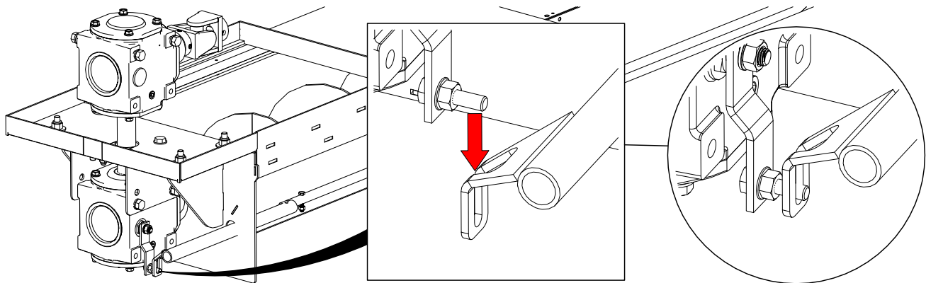
Figure 22. Slide Bolt through Shifter Linkage Slot
