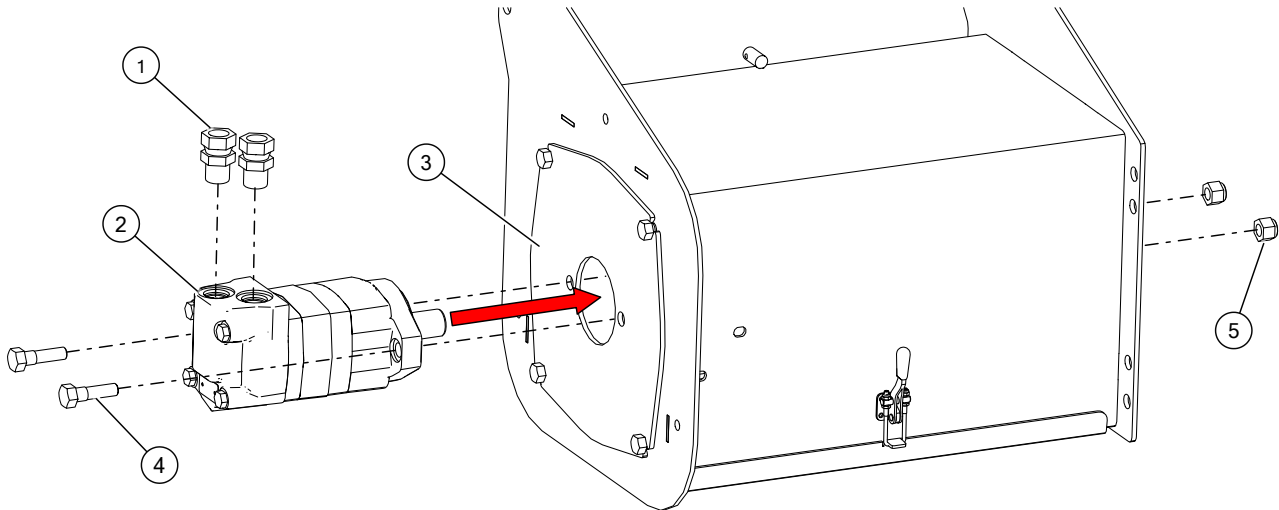
Figure 46. Mount Hydraulic Motor to Cover Plate
