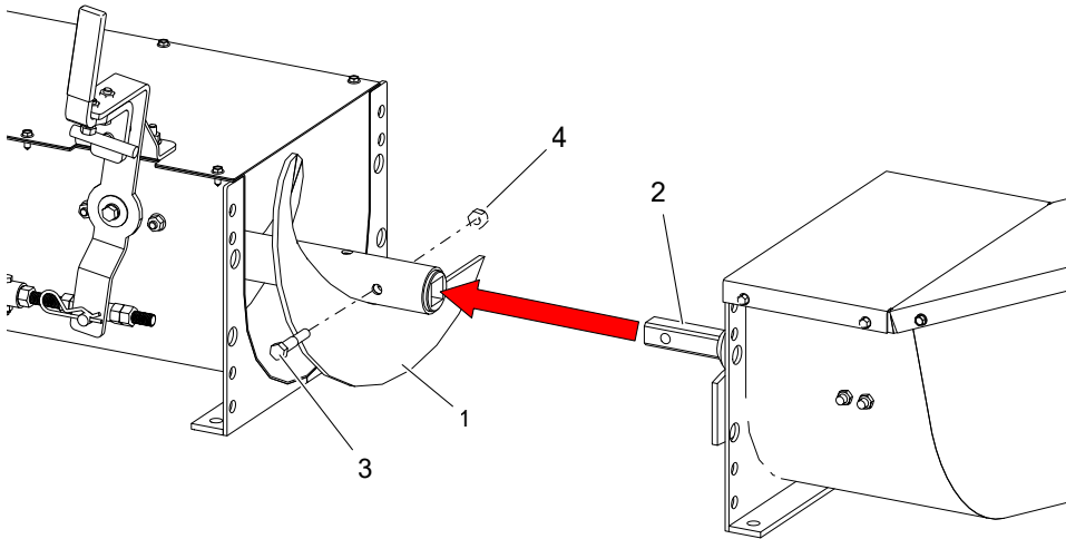
Figure 37. Install Transition Flighting
