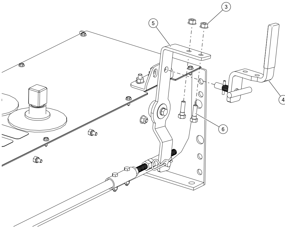
Figure 33. Assemble Gearbox Shift Handle
