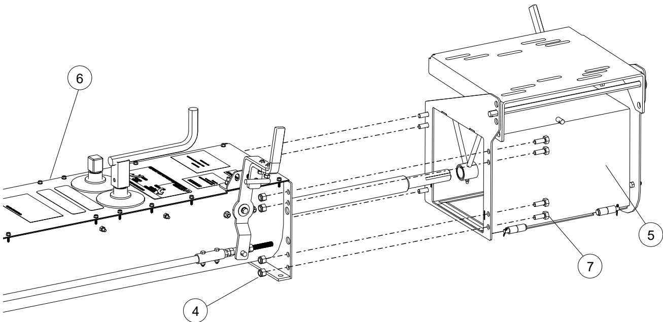
Figure 42. Mount Powerhead on the Underfloor Auger
